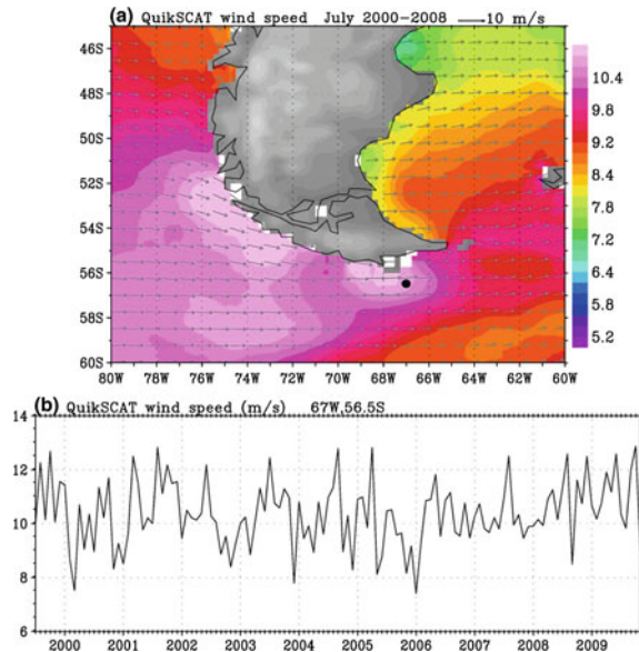
Fig. 15.7 Same as Fig. 15.6, except for a region around Tierra del Fuego
