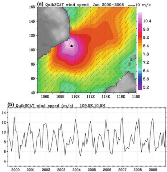
Fig. 15.11 Same as Fig. 15.6, except off the coast of Vietnam
