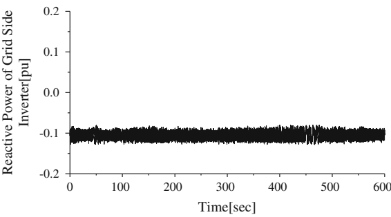
Fig. 6.27 Reactive power of grid side inverter
