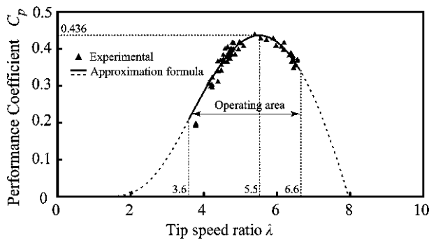
Fig. 5.12 C_p versus \lambda for the wind turbine
