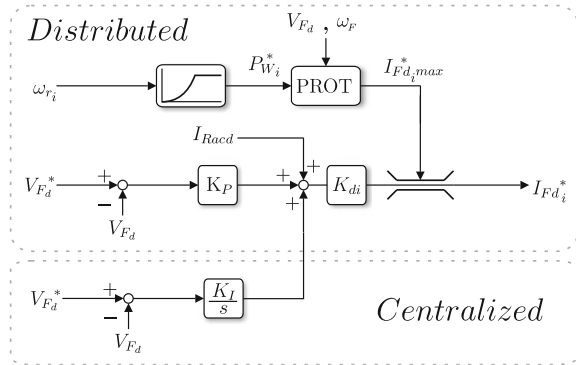
Fig. 18.7 Off-shore ac-grid voltage control
