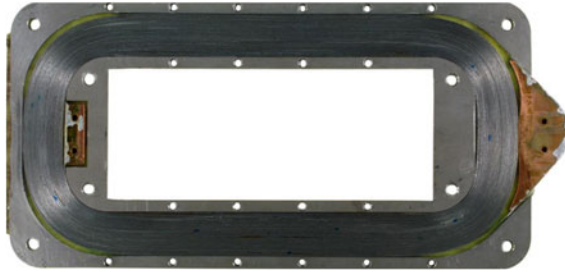
Fig. 3.13 High temperature superconducting race track coil holding 32 m of coated conductor from American Superconductor. The HTS tape is wound on an inner stainless steel frame with fiberglass tape inserted as insulation. Two copper blocks are used as current contacts and an outer stainless steel frame provides mechanical support for the winding. The coil is vacuum impregnated by epoxy after the winding. The dimensions of the coil are 240 \times 145 \times 5 mm and it was produced as part of the Superwind project [25]
