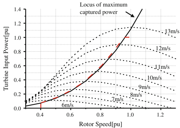
Fig. 6.15 Wind turbine characteristics for variable speed operation
