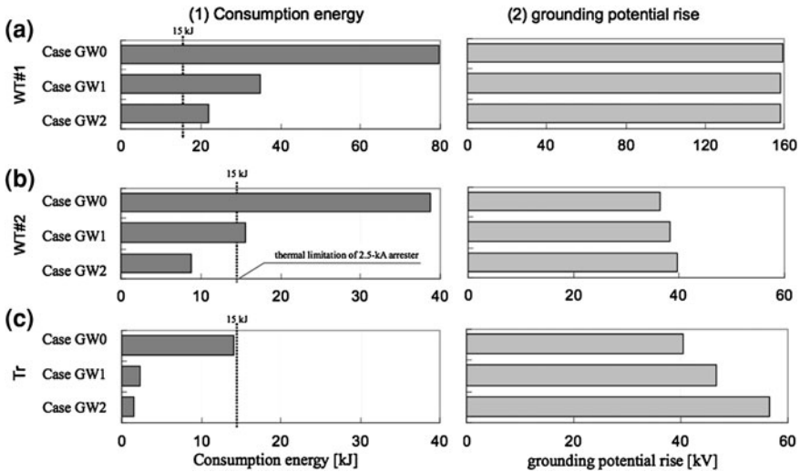
Fig. 11.16 Energy consumption at SPDs and maximum earth potential rise (EPR) at points around the wind farm in case of summer lightning ( 2/631 \mu\text{s} , 51 kA). (Column 1: total consumption energy at SPD, Column 2: maximum EPR, Row A: wind turbine No.1 (WT#1), Row B: wind turbine No.2 (WT#2), Row C: grid-interactive transformer (Tr).)
