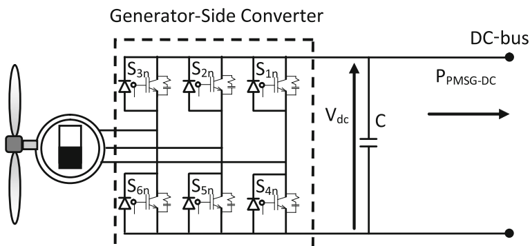
Fig. 21.5 Electrical scheme of the VSWT-PMSG
