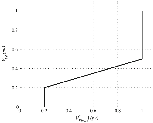
Fig. 18.12 VDCOL protection characteristic
