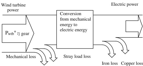
Fig. 2.6 Expression of power flow in the proposed method
