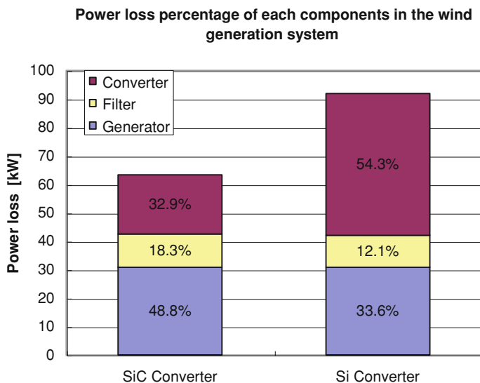
Fig. 4.15 Average power losses of SiC and Si wind turbine systems operating at full power rating and 3 kHz switching frequency
