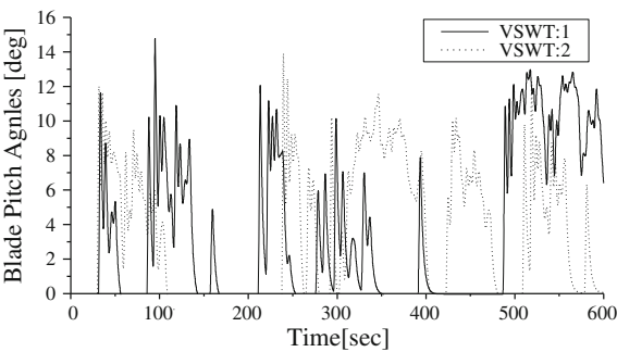
Fig. 21.16 Blade pitch angle of the wind turbines
