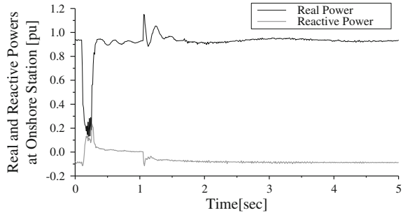
Fig. 21.23 Real and reactive powers at the onshore HVDC station (3LG)
