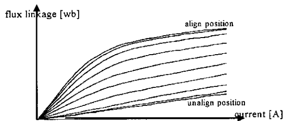
Fig. 6.4 The magnetization curves of SRM
