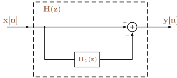
Fig. 8.12 The narrow band-pass filter scheme
