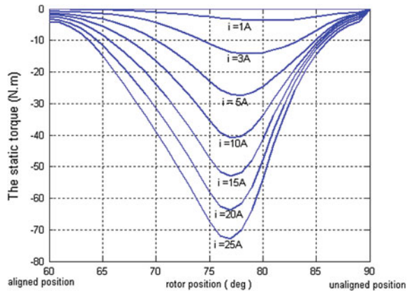
Fig. 6.11 The static torque curves of SRG
