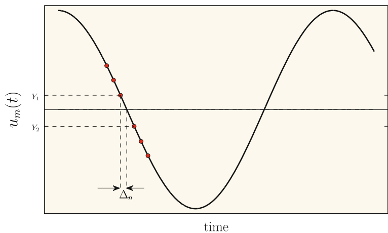
Fig. 8.9 The zero-crossing detection scheme
