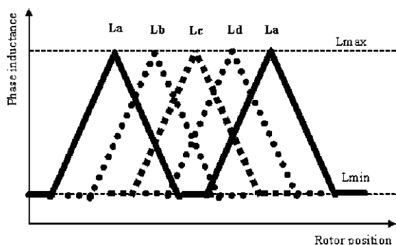
Fig. 6.7 The idealized phase inductance of a 4-ph 8/6 SRG
