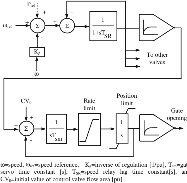
Fig. 14.7 Thermal and nuclear governors [24]
