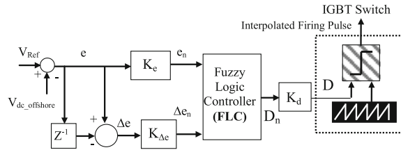
Fig. 21.8 Control block of the DC–DC buck/boost converter
