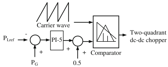
Fig. 14.12 The control concept of SMES charging and discharging mode
