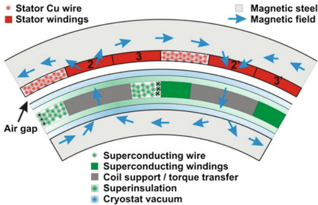
Fig. 3.9 Third generation direct drive generator based on superconducting rotor windings (green) embedded in multilayer thermal insulation material inside an evacuated cryostat. The cryostat is lying on the magnetic steel of the rotor, but the torque on the superconducting coils is transferred by a coil support structure inside the cryostat. The 3-phase stator winding is outside the cryostat and is kept at room temperature in order to be able to remove the heat from the copper windings. There are no magnetic steel teeth between the stator windings, because the air gap magnetic field is higher than the saturation limit of the steel. There would however typically be non-magnetic thin structural teeth to support the airgap stator winding. The outer steel ring is confining the flux in the generator and the losses will remain relatively low due to the low rotation speed
