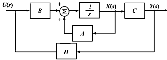
Fig. 16.7 Block diagram of the studied system with the designed damping controller (©2010 IEEE. Reprinted from IEEE Trans. Power Delivery , vol. 25, no. 2, April 2010)
