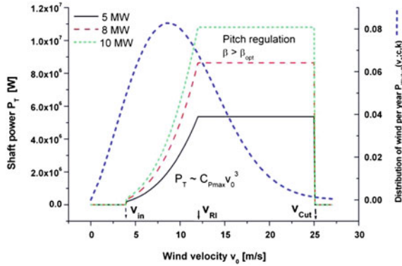
Fig. 3.2 Power curve of a Multibrid 5 MW turbine scaled to 8 and 10 MW by increasing the swept area of the rotor. The shaft power scales with the wind speed by v^3 up until the rated wind speed, where pitching of the turbine blades is used to limit the shaft power at the rated production. The blue curve represents the Weibull distribution of the wind power in the North Sea and the annual energy production of the turbine is determined by the integral of the product of the Weibull distribution and power curve [3]. Reproduced with permission from Institute Of Physics
