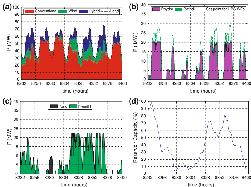
Fig. 13.3 Medium-size island system with an HPS. Operation during a typical week. a Output power of conventional units, hydro turbines and wind farms. b Output of HPS hydro turbines and wind farm. c HPS pump load and origin of pump energy. d Level of the HPS water reservoir, ([32], © [2009] IET)
