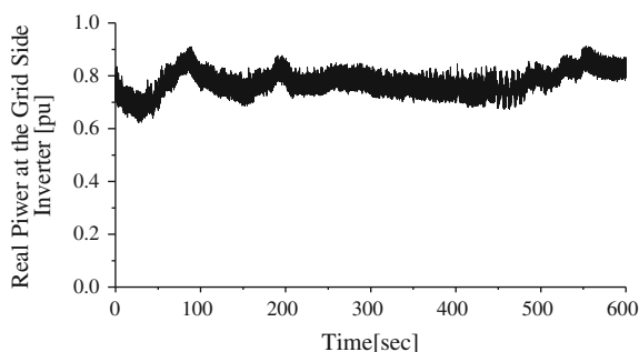
Fig. 6.26 Real power of grid side inverter
