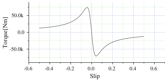
Fig. 2.5 Slip-torque curve
