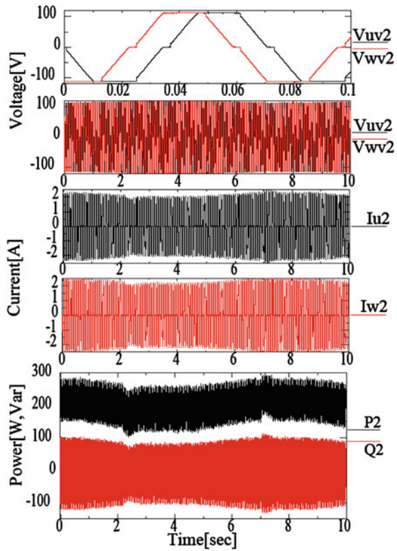
Fig. 20.9 Experimental results for coreless generator (offshore-wind turbine) voltages ( V_{uv2} & V_{vw2} ), currents ( I_{u2} & I_{w2} ), active power ( P2 ), and reactive power ( Q2 )
