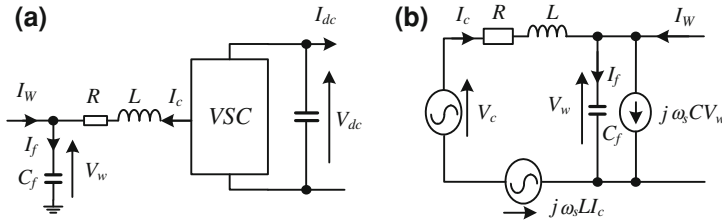
Fig. 17.5 Equivalent circuit of the WFSVC. a Schematic diagram. b ac equivalent circuit
