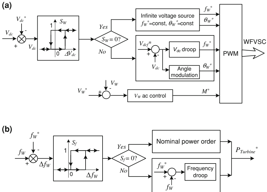
Fig. 17.10 System control for the WFVSC and wind farm for Option 2. a WFVSC control switch during grid fault (Option 2). b Wind turbine frequency control during fault
