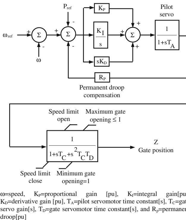
Fig. 14.6 Hydro governor [23]
