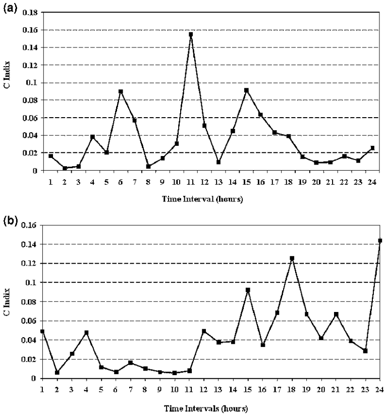
Fig. 9.7 C Indices for the developed models using the traditional GM(1,1). a Sample 1. b Sample 2
