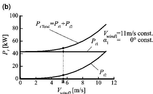
P_{t1} , P_{t2} versus V_{wind2} .
