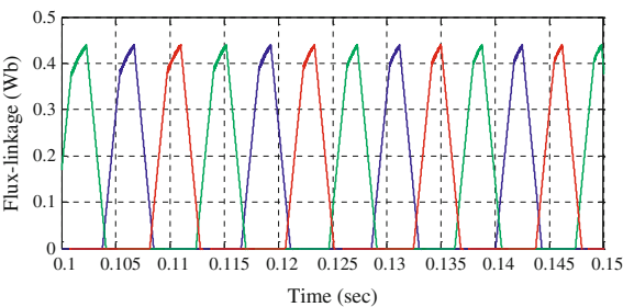
Fig. 6.17 The flux-linkage response of the SRG under \theta_{on} = 10^\circ and \theta_{off} = 30^\circ
