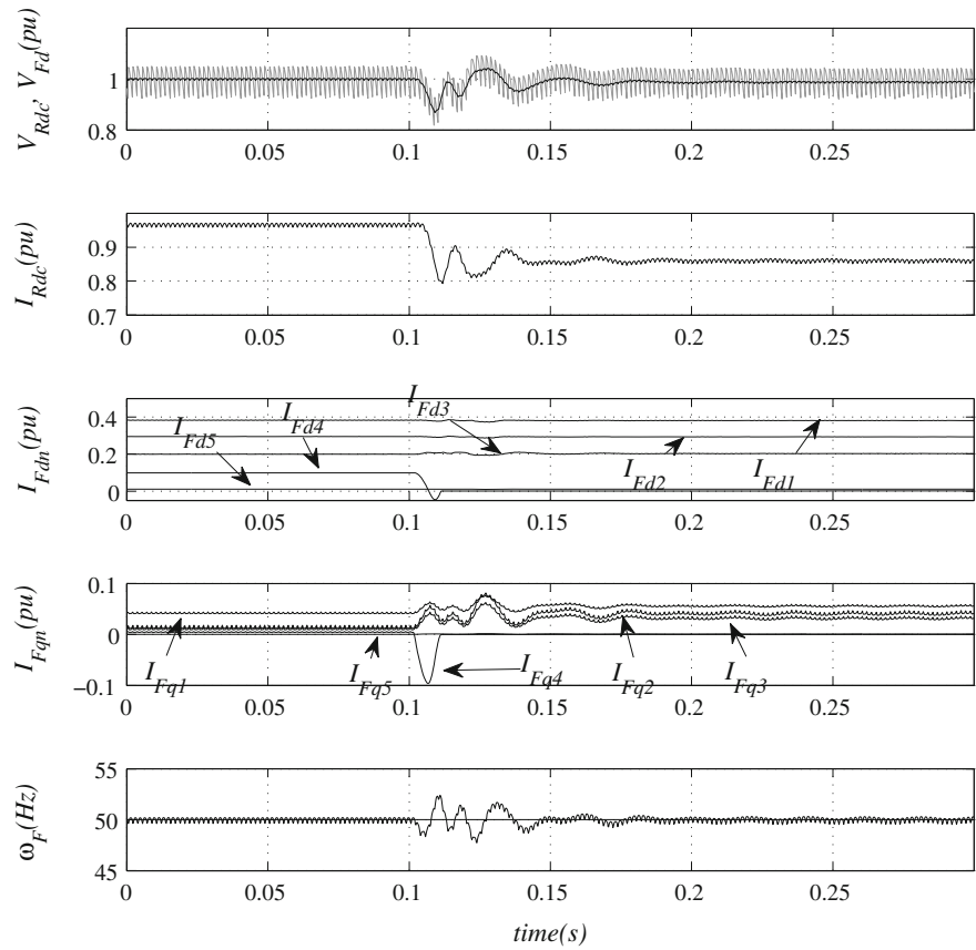
Fig. 18.20 Response to a sudden disconnection of 10% of the wind turbines
