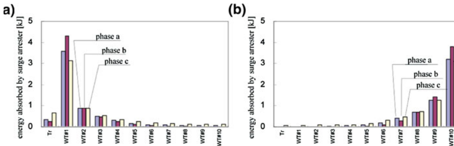
Fig. 11.7 Energy absorbed by SPDs in each wind turbine (Summer lightning R_{g0} = 6.77 \Omega ). a Case 1: Lightning on WT#1. b Case 2: Lightning on WT#10
