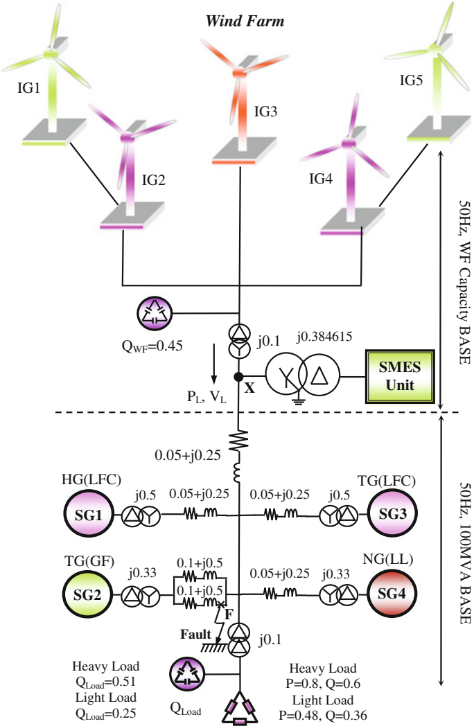
Fig. 14.5 Model system
