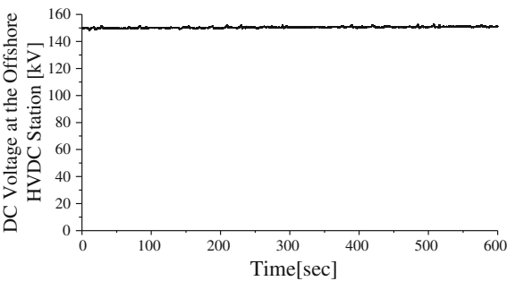
Fig. 21.18 Output voltage of the FB DC-DC converter
