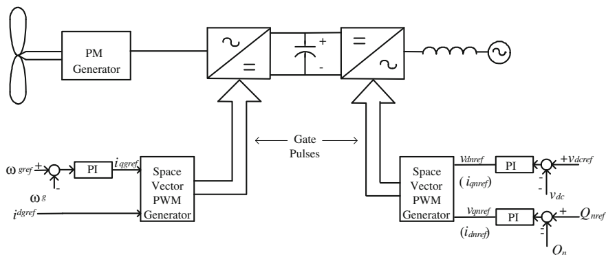
Fig. 7.8 Overall study system including the power and control sub-systems
