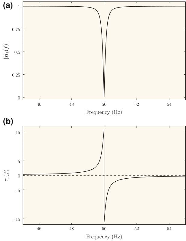
Fig. 8.11 Frequency responses of the notch filter. a Frequency response module of the notch filter. b Phase delay of the notch filter
