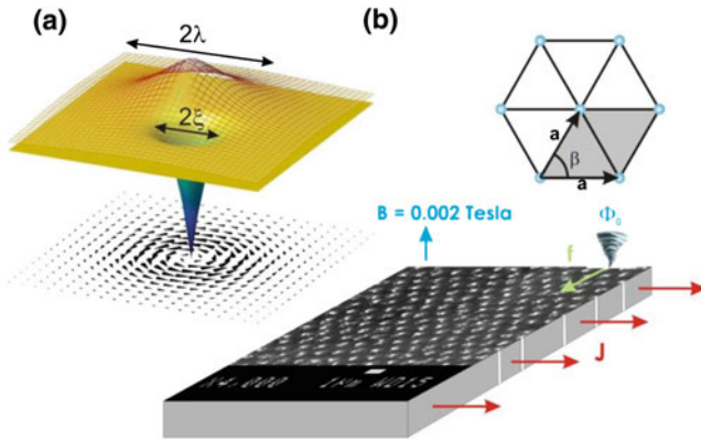
Fig. 3.10 a A flux line in a superconductor is a tube-shaped region where a circulating super current ( arrows ) are confining a quantum of magnetic flux \Phi_0 . The magnetic field distribution ( mesh ) and the supercurrent are decaying exponentially with the penetration depth \lambda . The density of the superconducting condensate ( surface ) is suppressed at the centre of the flux line in the normal core having a size given by the coherence length \xi . b Bitter decoration image of flux line lattice formed in a \text{TmNi}_2\text{B}_2\text{C} superconductor exposed to an applied field of B = 2 \text{ mT} . It should be noticed that the distance between the flux lines is about a = 1 \text{ }\mu\text{m} , which is large compared to \lambda = 80 and \xi = 15 \text{ nm} [18]. A force f perpendicular to the flux line \Phi_0 results if a transport current density J is applied to the superconductor and dissipation is caused if the flux lines moves
