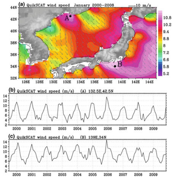
Fig. 15.18 Same as Fig. 15.6, except for a region around Japan
