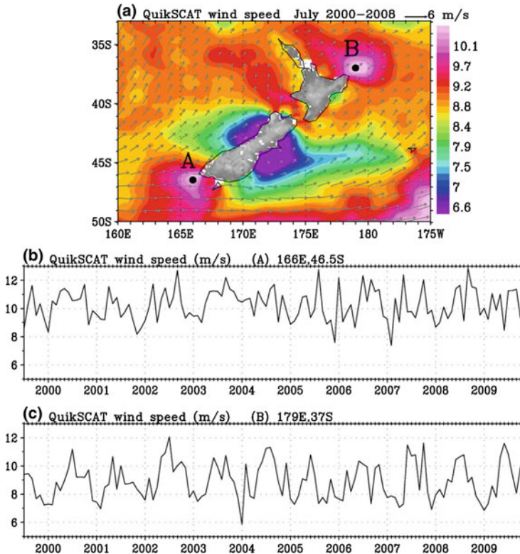
Fig. 15.6 (a) Wind speed (color) averaged for July from nine years of QuikSCAT data (2000–2008), with superimposition of QuikSCAT equivalent neutral wind vectors (arrows) for the same period, around New Zealand. (b) and (c) are time series of monthly mean wind speed at two selected locations marked in (a)
