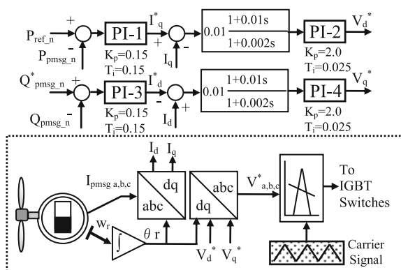
Fig. 21.5 Electrical scheme of the VSWT-PMSG
