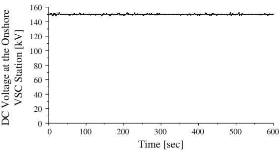
Fig. 21.19 DC voltage of the onshore HVDC station
