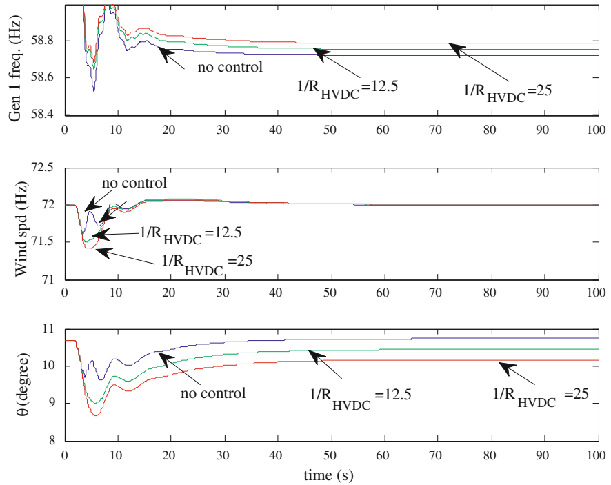
Fig. 19.8 Dynamic responses of the speed of Generator 1, the rotating speed of wind turbine, and blade angle
