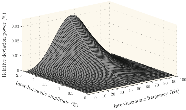
Fig. 8.6 Relative error power between the estimated voltage and the reference voltage in case of the STFT technique
