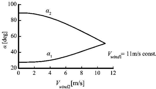
Fig. 5.9 Control angles \alpha_1 , \alpha_2 versus V_{\text{wind } 2} for the case with constant load resistance
