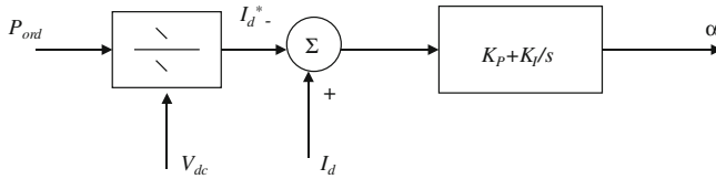
Fig. 19.1 Current control scheme at an HVDC's rectifier
