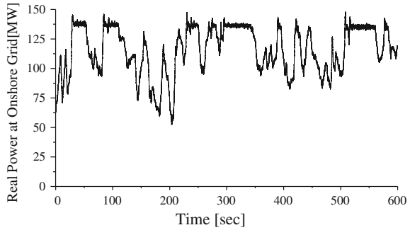
Fig. 21.21 Real power at the onshore grid
