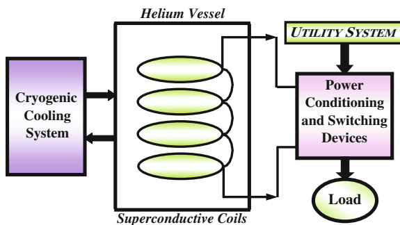
Fig. 14.4 Schematic diagram of the basic SMES system
