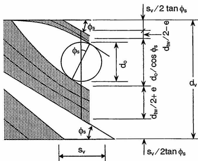
Figure 2.17 Truss action in beam with opening.
