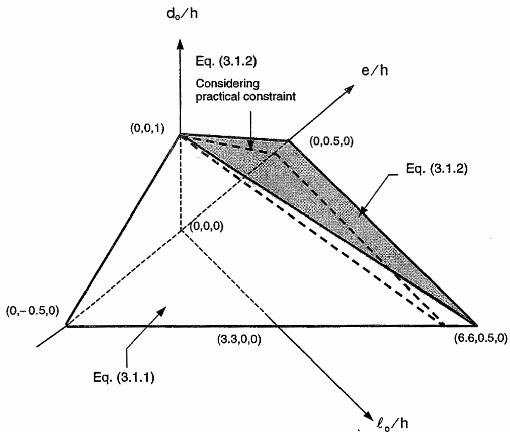
(b) Domain of (\ell_o, d_o, e) for which slenderness effect in compression chord can be ignored
