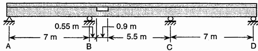
(a) Continuous beam with opening
