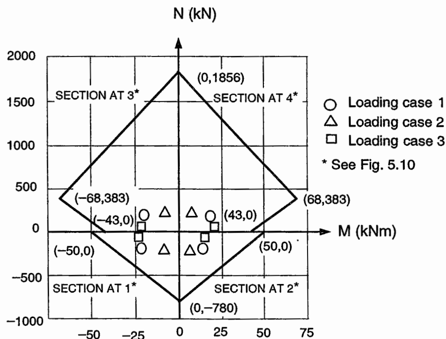
Figure E5.1.5 Linearized interaction diagrams for chord members.
