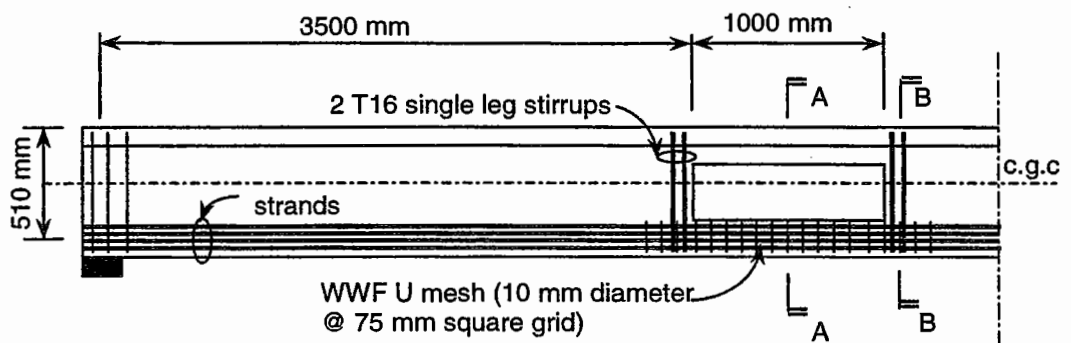
(a) Elevation
