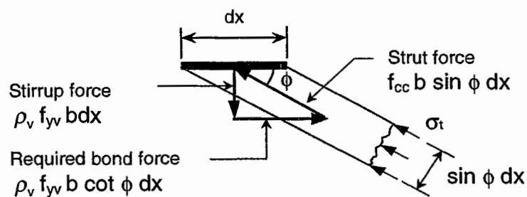
(a) Analogous truss model
