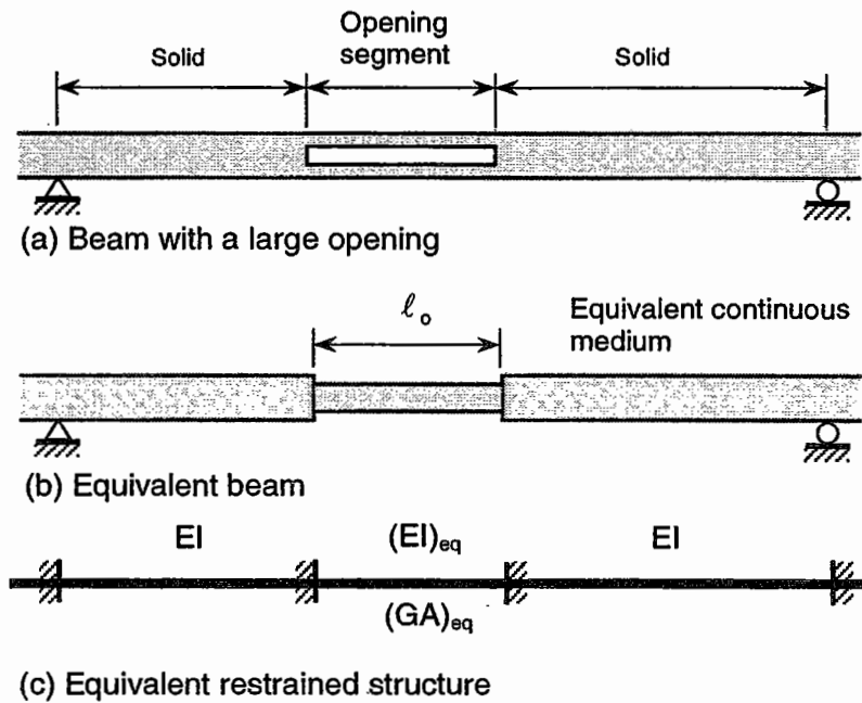
Figure 5.3 Equivalent segmented beam.
