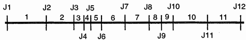
(c) Equivalent segmented beam for service load analysis
