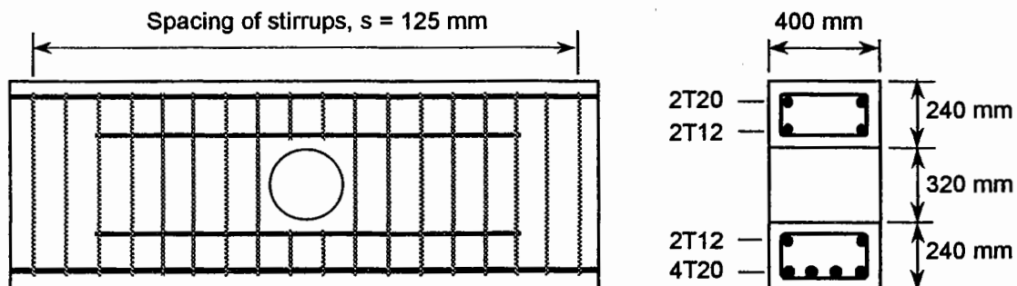
Figure E2.5.1 Reinforcement details of beam.
