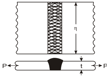
Single V-Butt joint
