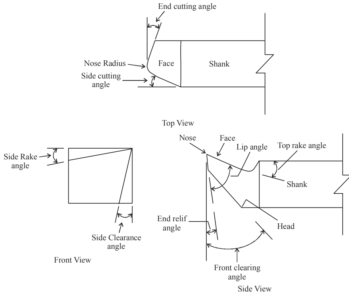
Cutting Tool Angles
