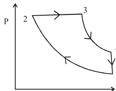
Diesel Cycle
