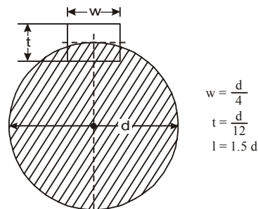
Rectangular sunk key
