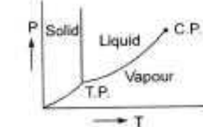
Fig. (b) p-v-T surface of a substance which contracts on freezing
