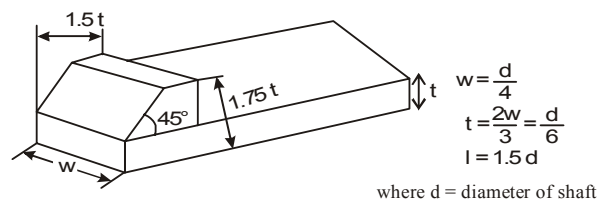
Gib head sunk key
