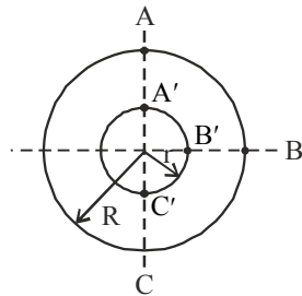
Cross-section of a shaft at free end
