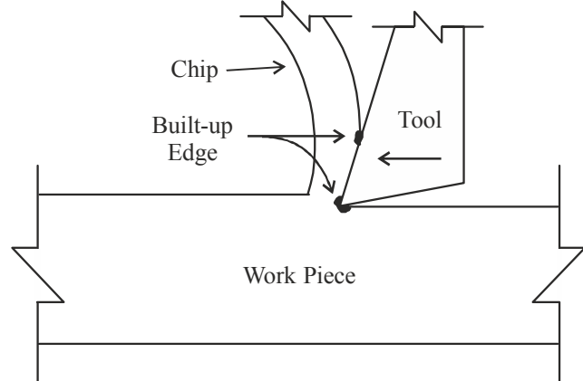
Showing Built-up edge
