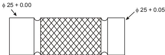
Fig. Plug gauge
