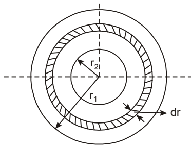
Disc clutch
