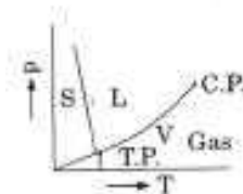
Fig. (a) p-v-T surface for water which expands a freezing
