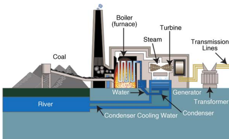
Figure 2.14 Conventional fossil-fuel generation (Source: http://commons.wikimedia.org/wiki/File:Coal_fired_power_plant_diagram.svg )
