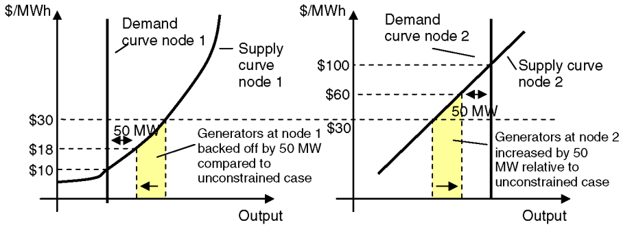
Figure 7.3 A two-node network with a constrained link
