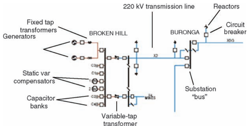
Figure 2.20 Schematic diagram of the electricity transmission network in the Broken Hill region (Source: From AEMO documents)
