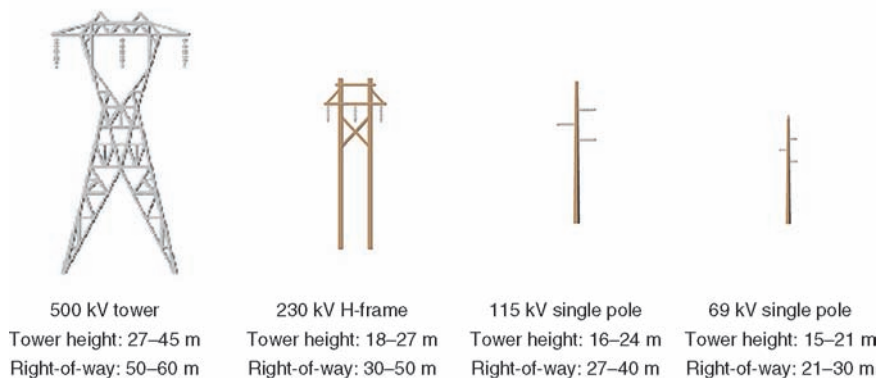
Figure 2.18 Dimensions of transmission towers of different voltages (Source: Minnesota Electric Transmission Planning at http://www.minnelectrans.com/transmission-system.html )
