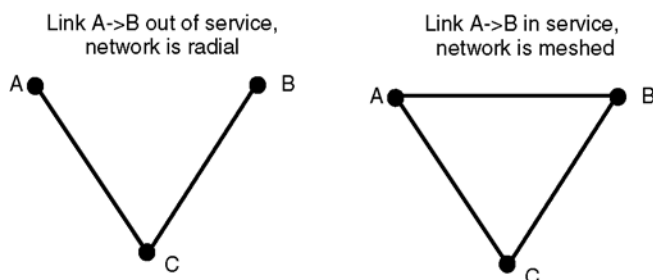
Figure 8.1 Alternative network configurations
