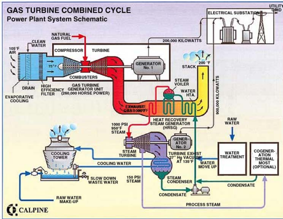
Figure 2.15 Combined-cycle gas turbine (Source: http://www.power-technology.com/projects/san_joaquin/san_joaquin3.html )
