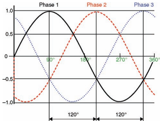
Figure 2.12 The movements of voltage and current in three-phase power (Source: http://commons.wikimedia.org/wiki/File:3_phase_AC_waveform.svg )
