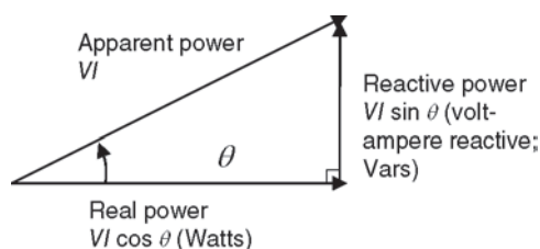
Figure 2.9 Schematic relationship between real, reactive and apparent power
