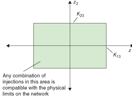
Figure 6.3 The set of feasible injections in a simple two-link network
