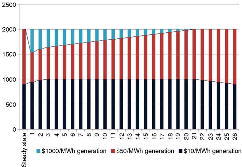
Figure 11.2 Optimal dispatch ignoring the contingency
