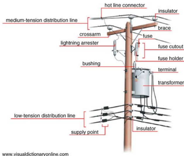
Figure 2.21 Typical distribution network assets (Source: http://visual.merriam-webster.com/energy/hydroelectricity/electricity-transmission/overhead-connection.php )
