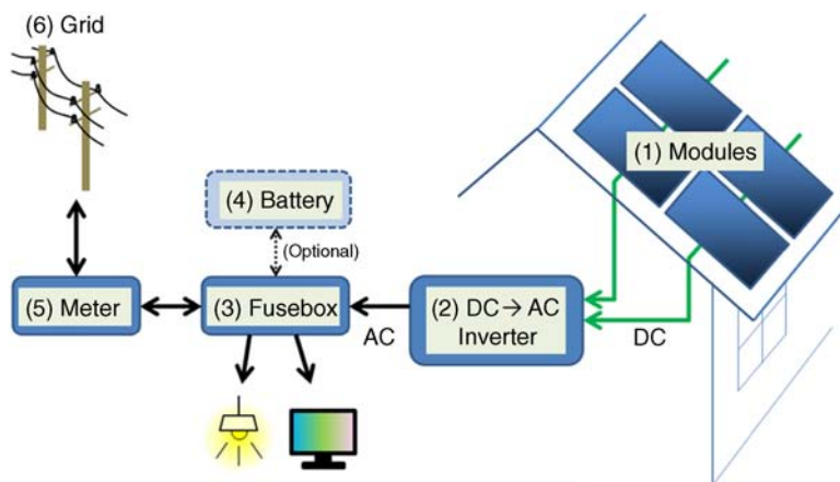
Figure 2.16 Typical simple solar PV installation (Source: http://commons.wikimedia.org/wiki/File:PV-system-schematics-residential-Eng.png )
