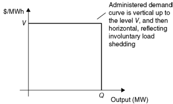
Figure 5.4 Effective demand curve in the presence of unresponsive load and an administered price cap
