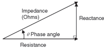
Figure 2.11 Schematic relationship between impedance, reactance and resistance in an AC circuit
