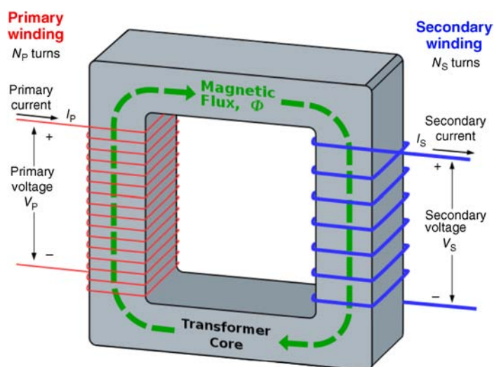
Figure 2.5 The transformation of the voltage in a transformer depends on the ratio of the number of turns (Source: http://en.wikipedia.org/wiki/File:Transformer3d_col3.svg )
