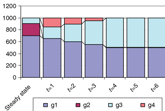
Figure 11.7 Optimal pre- and postcontingency dispatch in a simple meshed network with one binding transmission constraint
