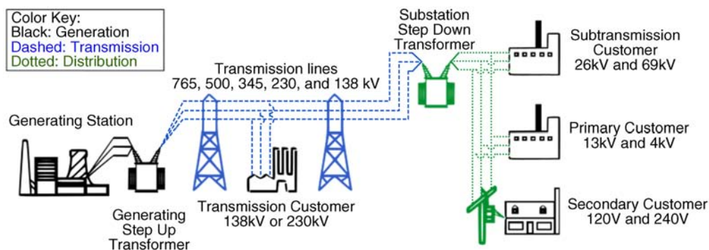
Figure 2.13 The basic elements of a power system (Source: http://en.wikipedia.org/wiki/File:Electricity_grid_simple-_North_America.svg )
