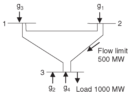
Figure 11.6 Simple three-node network diagram
