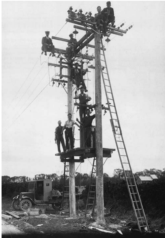
Construction of a pole-mounted transformer substation, Waitaki Electric Power Board, New Zealand, ca 1925 (Source: Neil Rennie, Power to The People: 100 Years of Public Electricity Supply in New Zealand , Electricity Supply Association of New Zealand)
