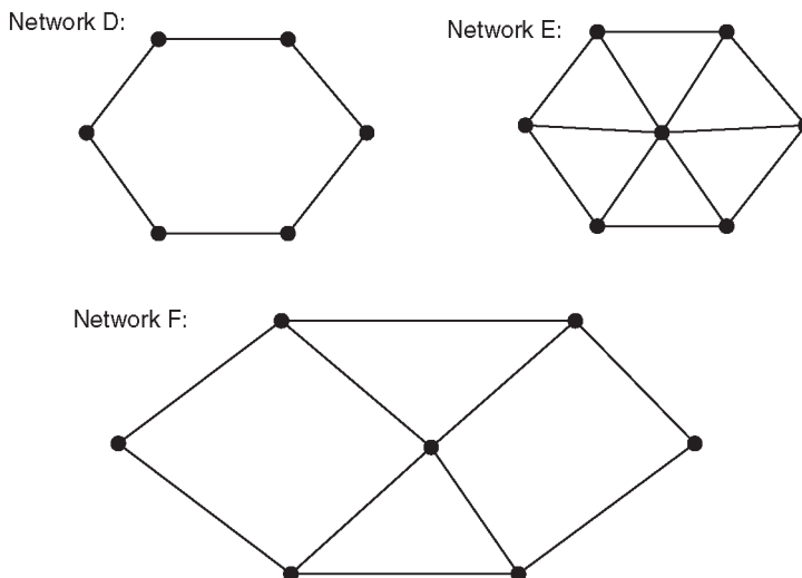
Figure 6.2 Examples of meshed networks
