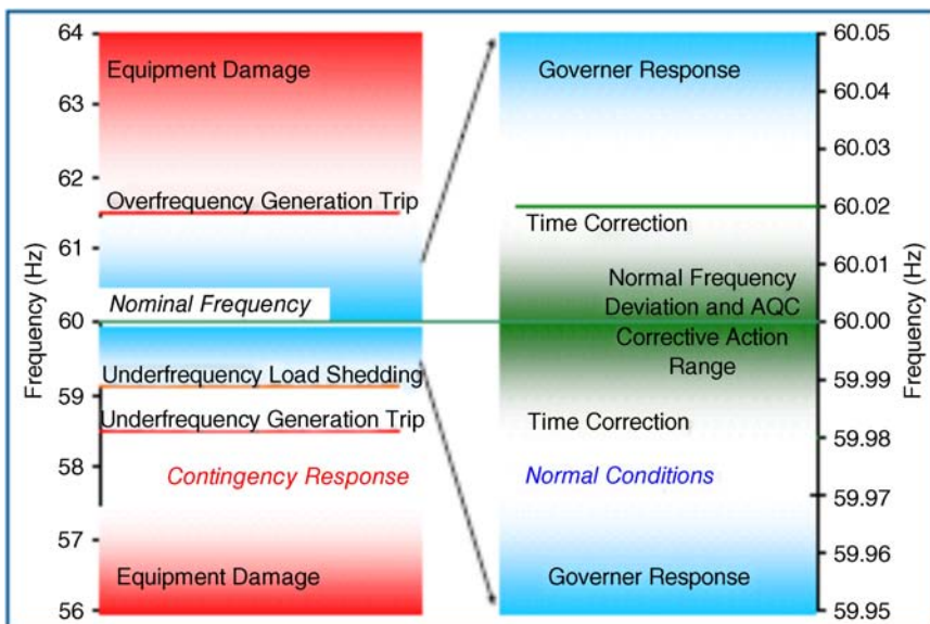
Figure 2.22 Normal frequency ranges for a 60 Hz power system (Source: Kirby, B., J. Dyer, C. Martinez, R. A. Shoureshi, R. Guttromson and J. Dagle, (2002), “Frequency Control Concerns in the North American Electric Power System”, prepared for the U.S. Department of Energy, ORNL/TM-2003/41, available at: http://web.ornl.gov/~webworks/cppr/y2001/rpt/116362.pdf )
