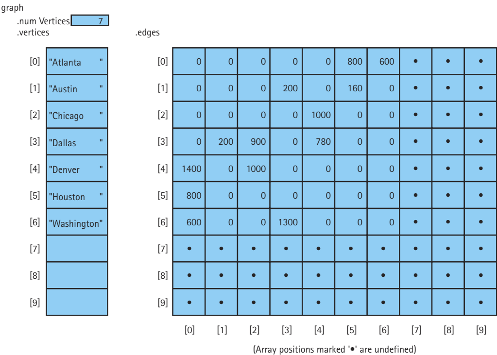
Figure 9.15 Graph of flight connections between cities
