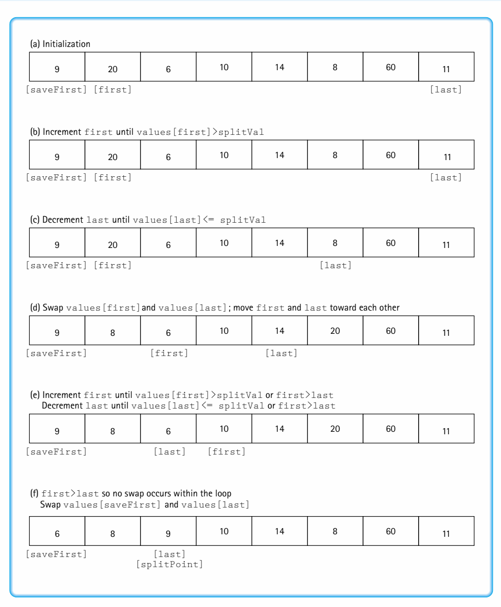
Figure 7.8 Function split
