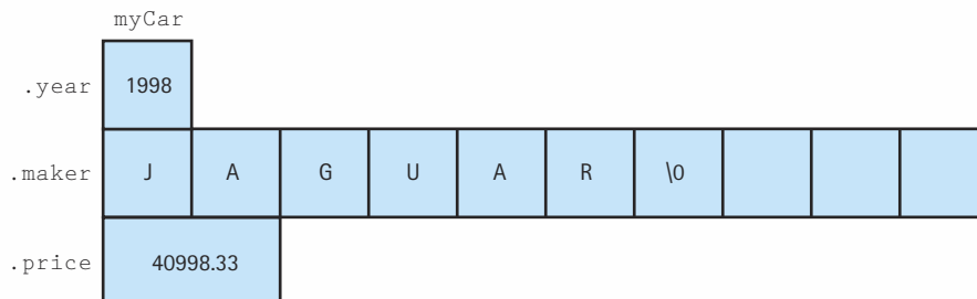
Figure 2.5 Record myCar
