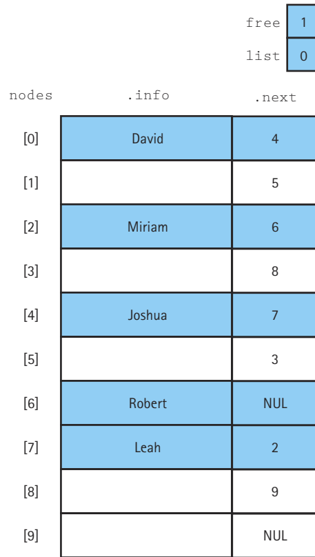
Figure 6.20 List and linked structure are together
