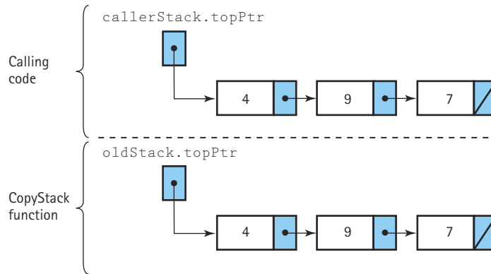
Figure 6.13 Shallow copy versus deep copy of a stack
