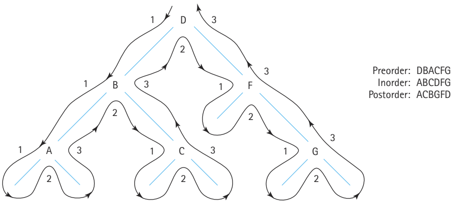
Figure 8.16 Visualizing binary tree traversals
