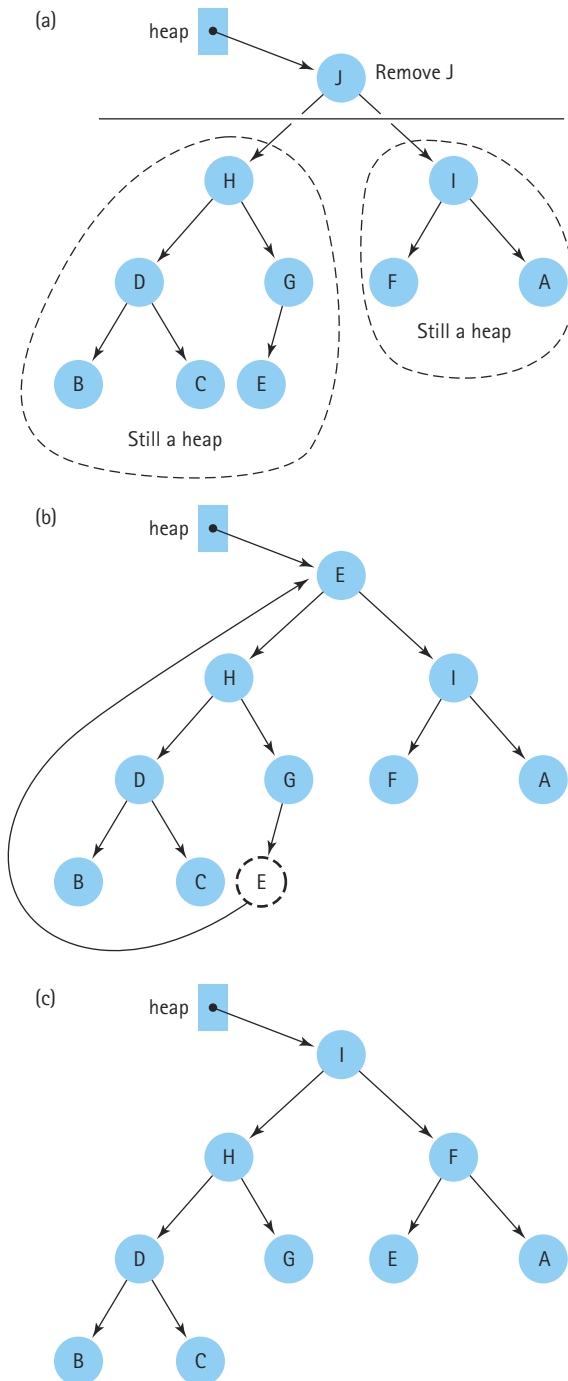
Figure 9.3 The ReheapDown operation
