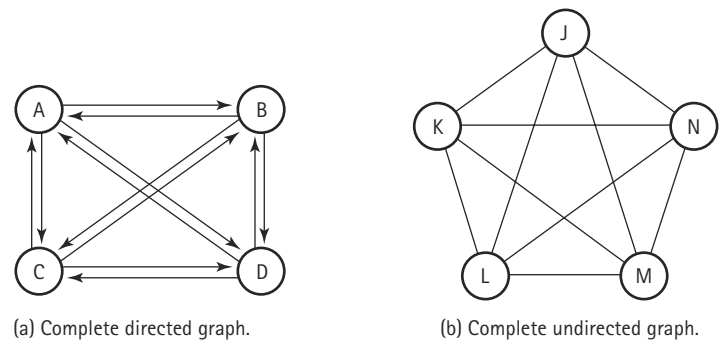
Figure 9.9 Two complete graphs
