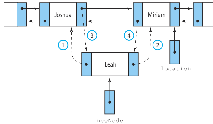
Figure 6.9 Linking the new node into the list
