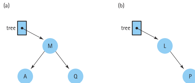
Figure 8.5 Two binary search trees
