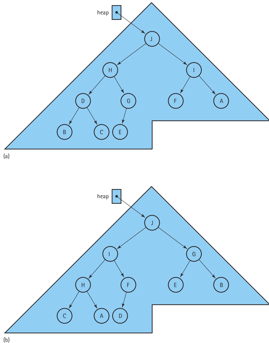
Figure 9.2 Two heaps containing the letters "A" through "J"
