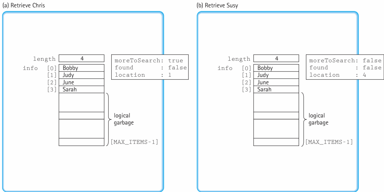
Figure 3.5 Retrieving in a sorted list
