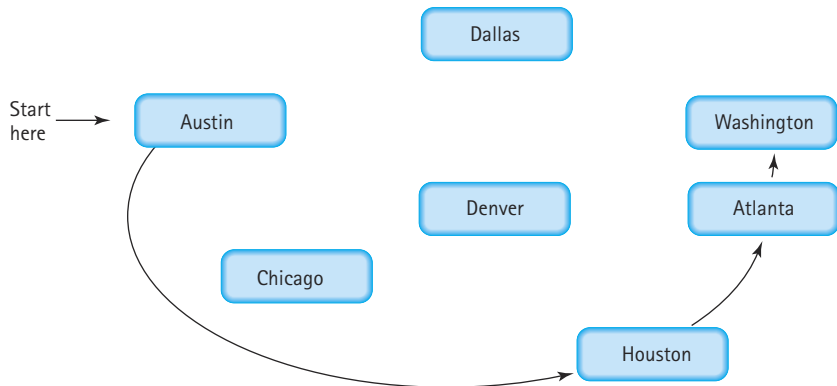
Figure 9.12 The depth-first search
