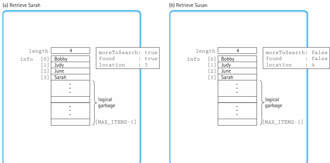
Figure 3.2 Retrieving an item in an unsorted list
