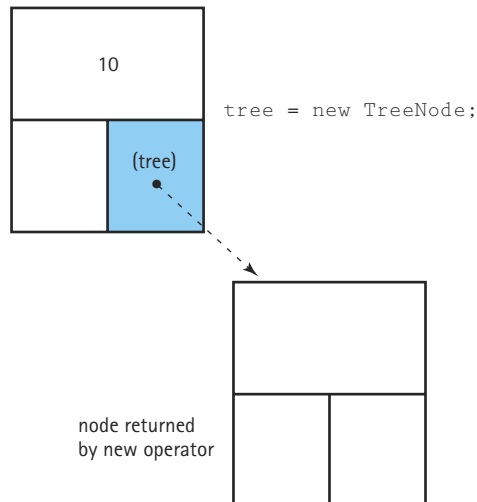
Figure 8.9 The tree parameter is a pointer within the tree
