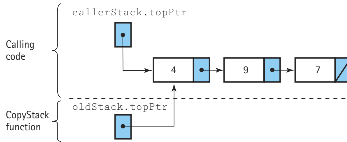
(a) A shallow copy
