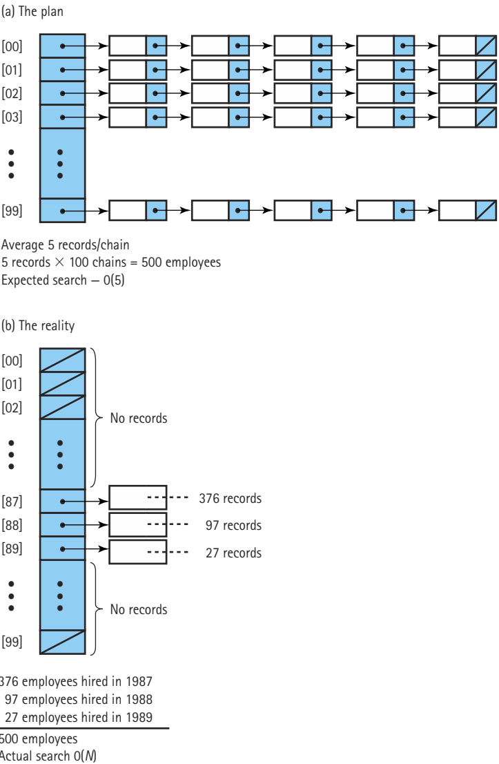
Figure 10.25 Hash scheme to handle employee records
