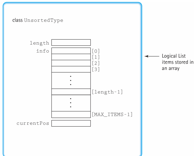
Figure 3.1 Data members of class UnsortedType
