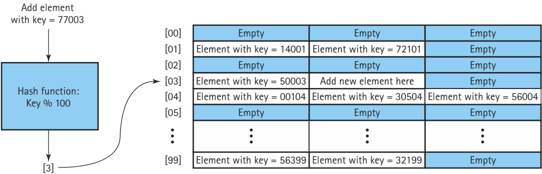
Figure 10.22 Handling collisions by hashing with buckets
