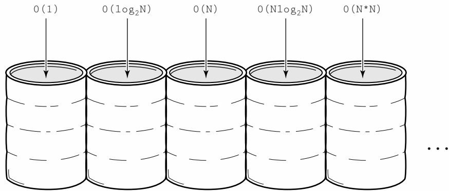
Figure 3.10 Complexity bins
