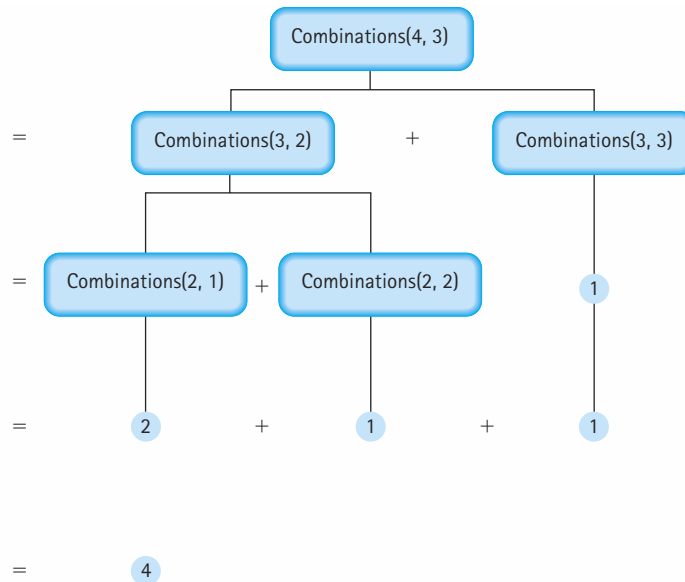
Figure 7.2 Calculating Combinations (4, 3)
