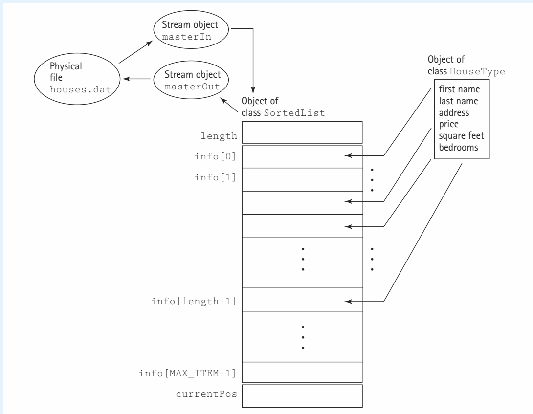
Figure 3.13 The data objects in the case study
