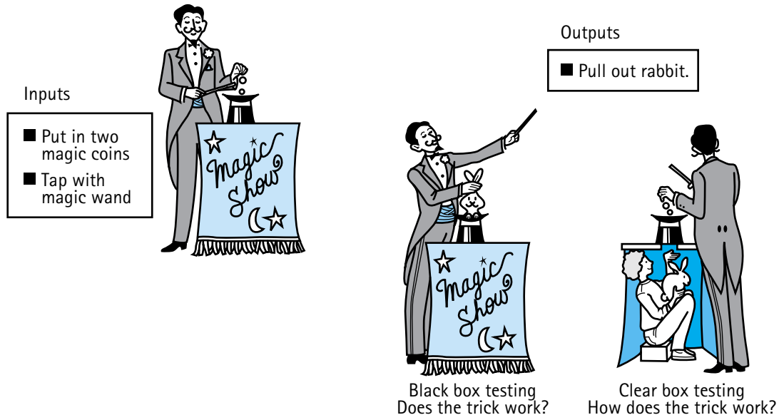
Figure 1.6 Testing approaches
