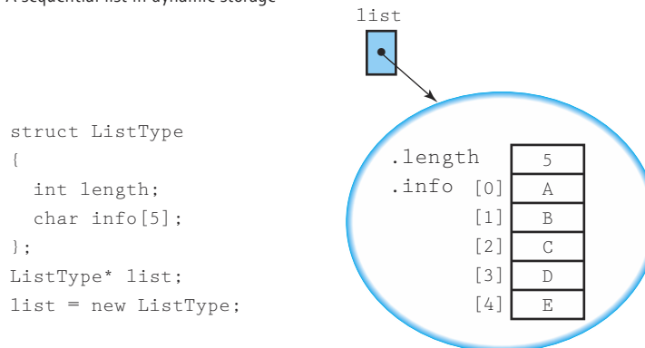
Figure 6.15 Array-based lists in static and dynamic storage
