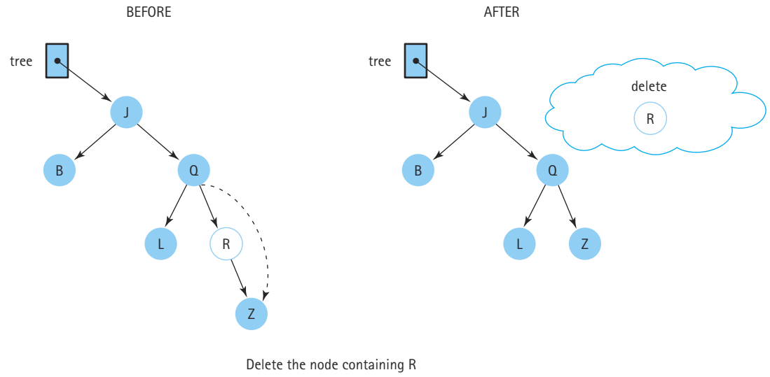
Figure 8.12 Deleting a node with one child
