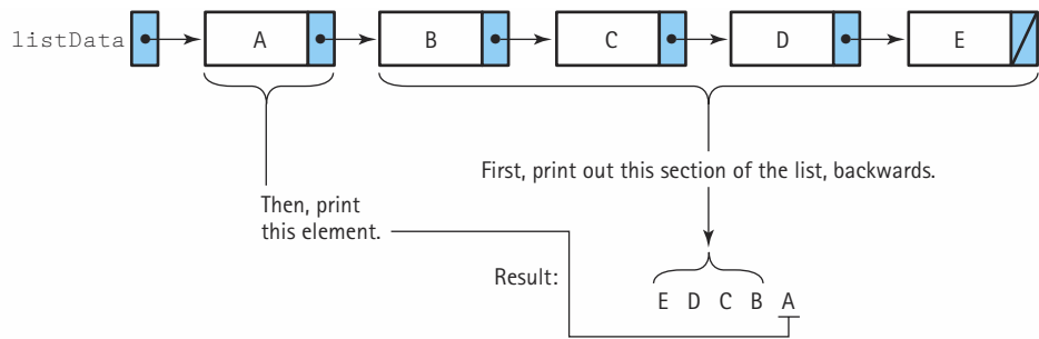
Figure 7.3 Recursive RevPrint
