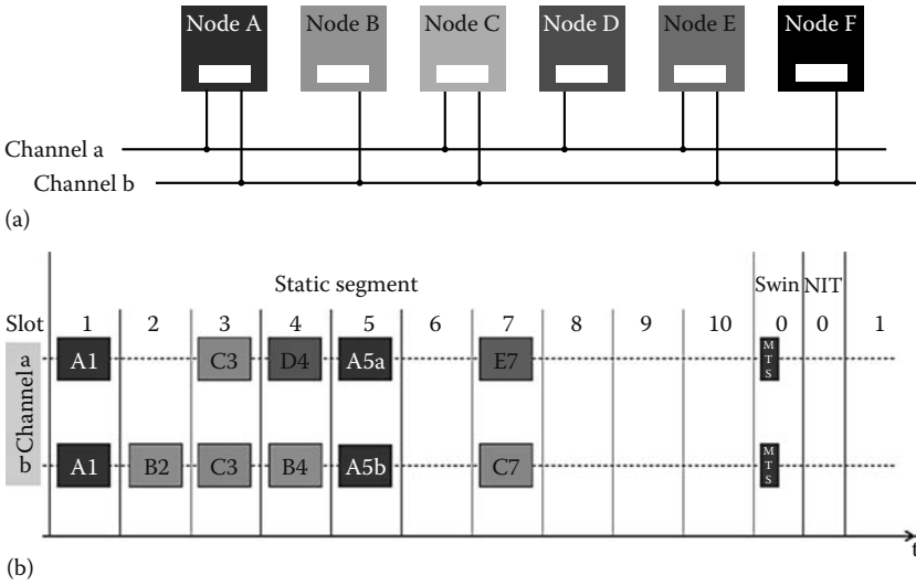
FIGURE 5.3 Example of communication in the static segment. (a) Sample cluster. (b) Frame transmissions in several static slots. (Copyright by DECOMSYS, Member of Elektrobitt. With permission.)
