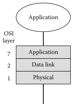
FIGURE 6.2 Communication architecture of a fieldbus device.
