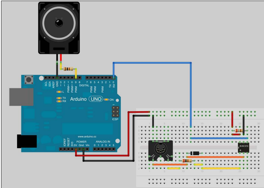
The MIDI-featuring sound generator based on Arduino
