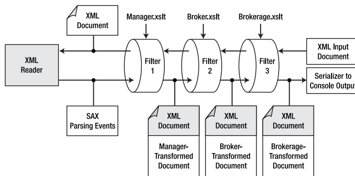
Figure 5-6. XSLT filtering
