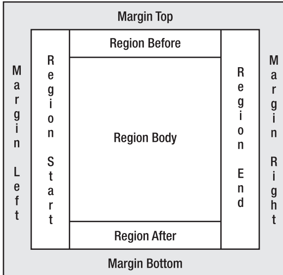
Figure 6-2. Page structure
