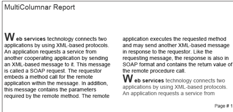
Figure 6-9. Two-column output
