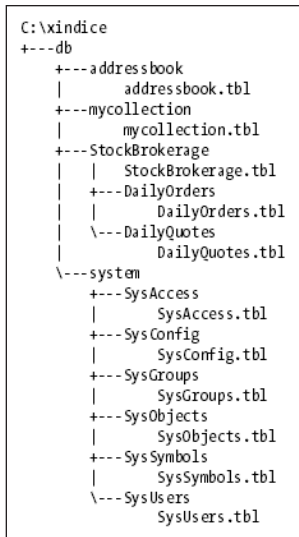
Figure 9-1. Xindice database structure
