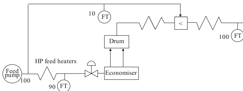
Figure 6.6 Cold spray
