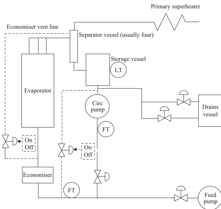
Figure 6.13 Sub-cooling and vent line
