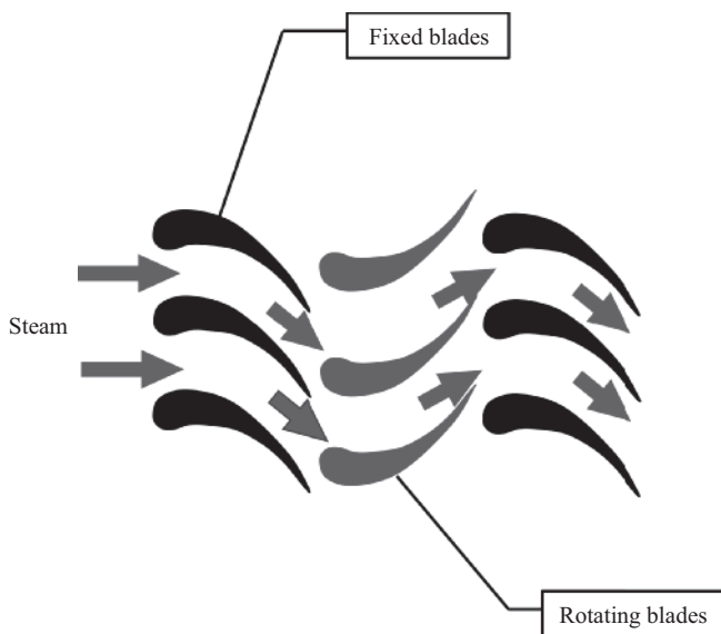
Figure 2.5 Turbine blading
