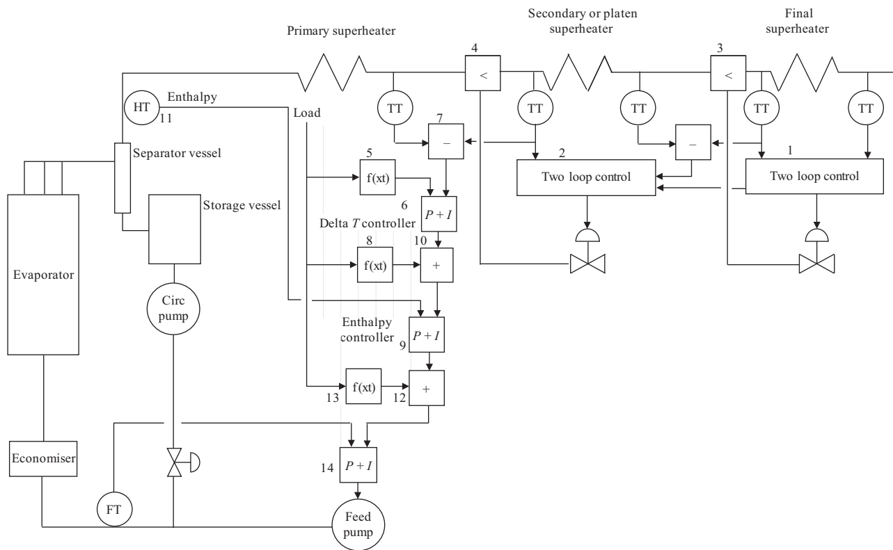
Figure 6.16 Basic enthalpy logic
