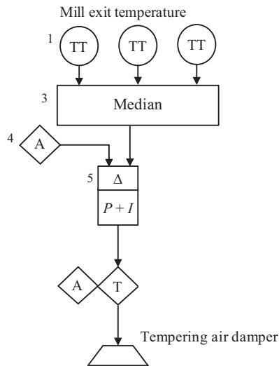
Figure 5.14 Simple mill exit temperature control for two-damper system
