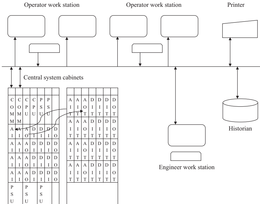
Figure 8.1 Generic DCS hardware configuration
