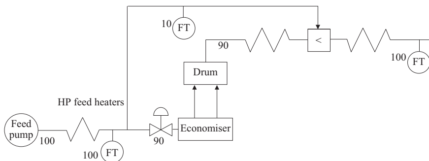
Figure 6.5 Hot spray
