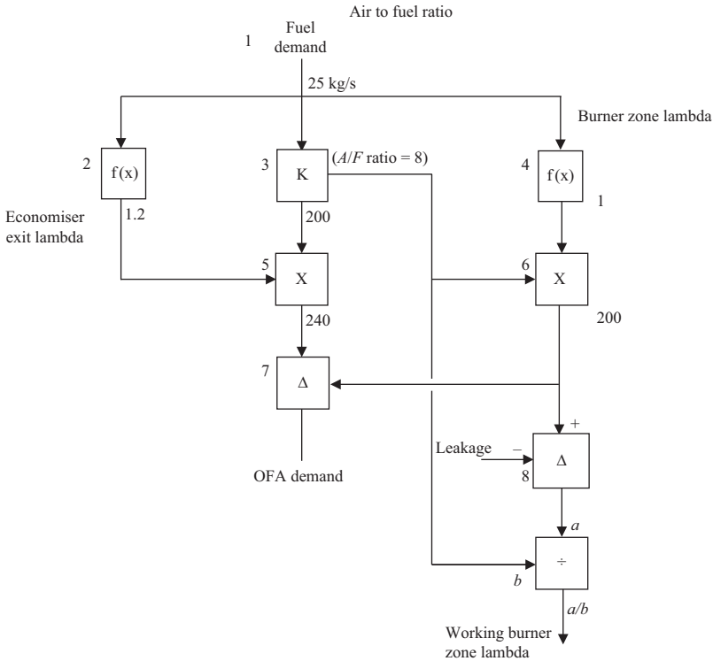
Figure 5.20 OFA logic. Based on Doosan Babcock technology and published with permission
