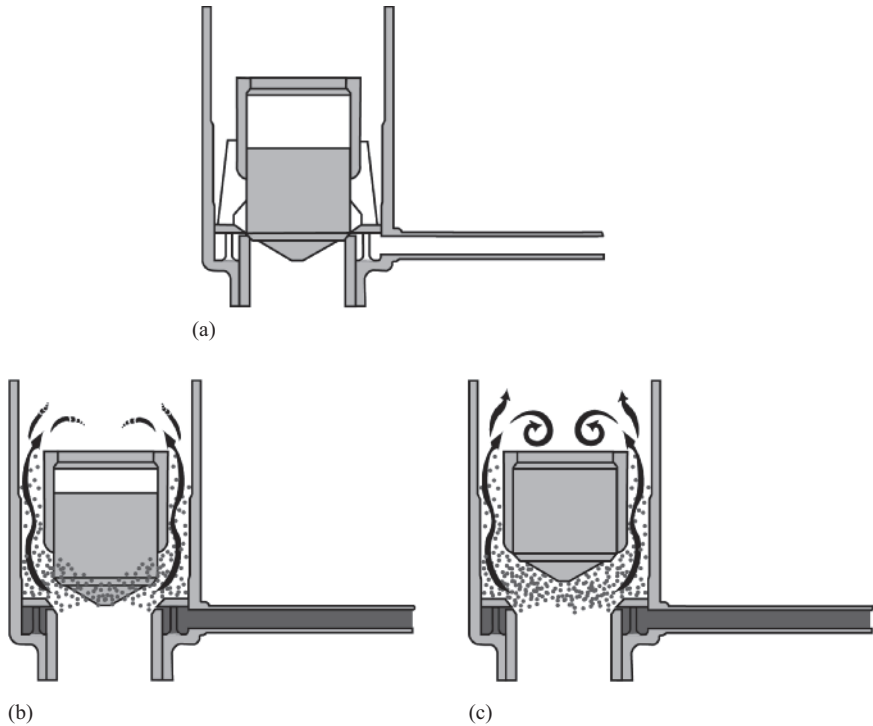
Figure 7.4 (a) No load variable orifice attenuator; (b) lightly loaded variable orifice attenuator; (c) variable orifice desuperheater at full load. © SPX Flow, reproduced with permission
