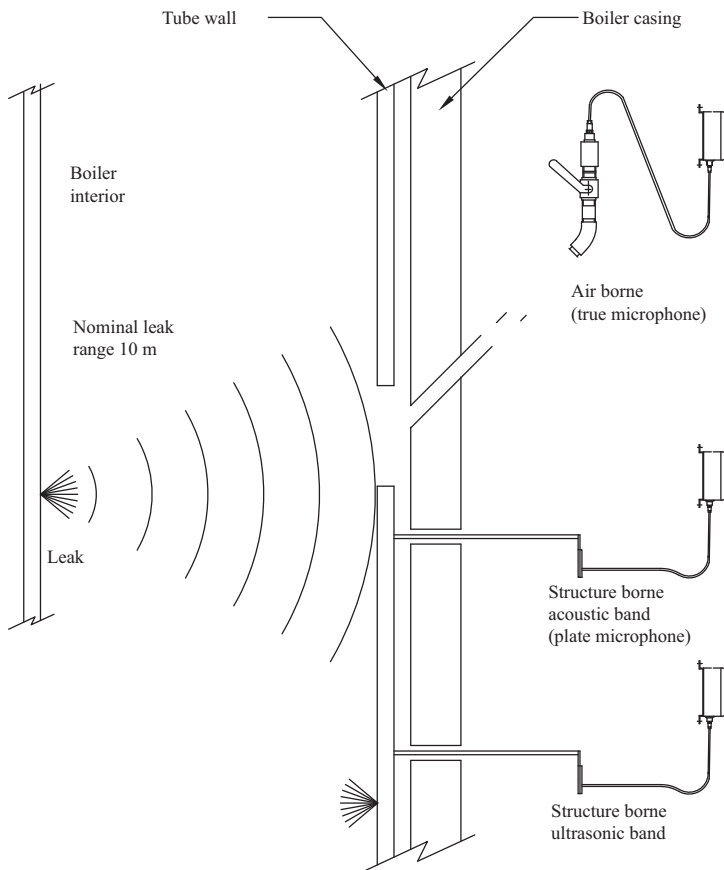
Figure 5.25 Acoustic probe assembly. © Procon Engineering, reproduced with permission
