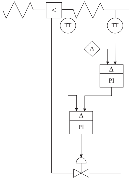
Figure 7.6 Steam temperature control with a single inter-stage spray attenuator
