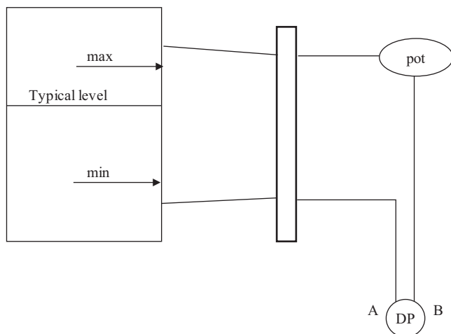
Figure 6.20 Drum-level measurement with a column
