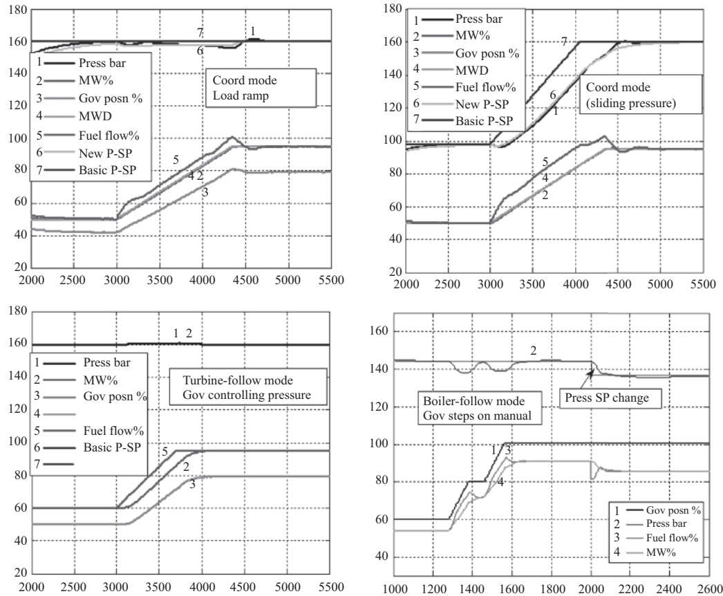
Figure 4.5 Simulations of load ramps in each control mode
