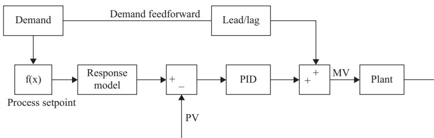
Figure 11.2 Two-degree-of-freedom feedforward/feedback control design
