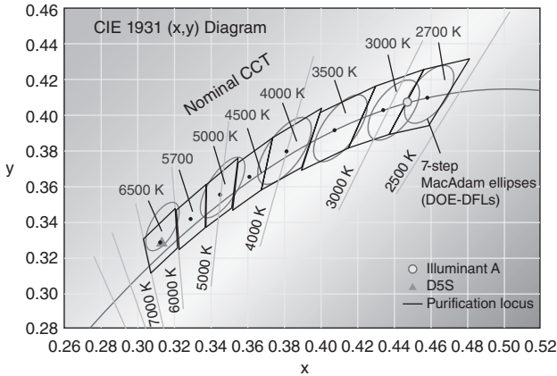
Figure 3.12 (x, y) Chromaticity Diagram Showing CCT and 7-Step MacAdam Ellipses. Source: http://www.photonics.com/Article.aspx?AID=34311 . See color insert.
