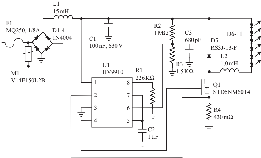
Figure 10.16 Final HV9910 Schematic for LED BR40.
