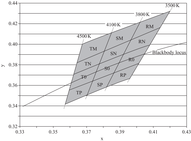
Figure 4.10 Neutral-White Bin Structure.
