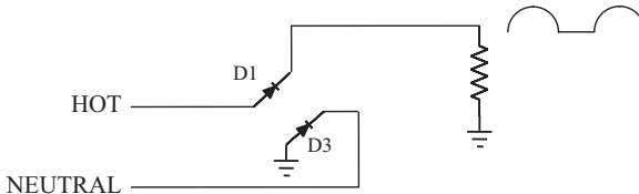
Figure 8.3 Half-Wave Rectification.
