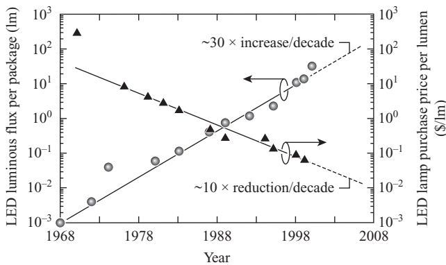
Figure 1.4 Haitz's Law.
