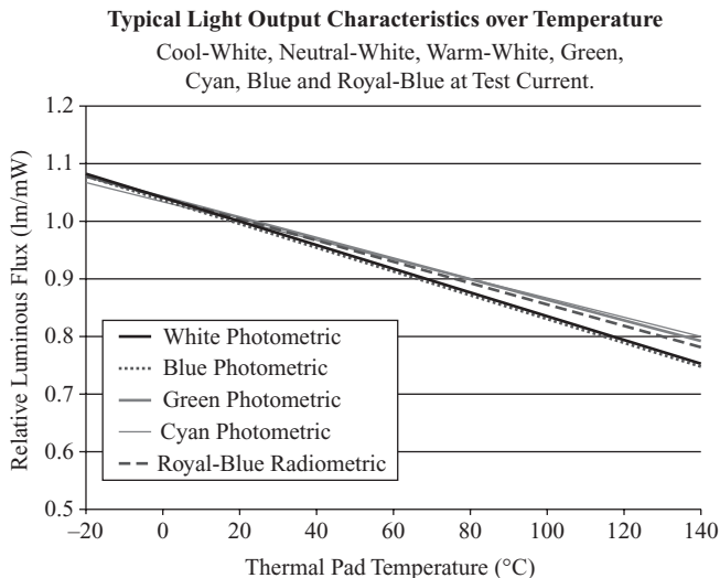
Figure 5.1 Brightness as a Function of Temperature.
