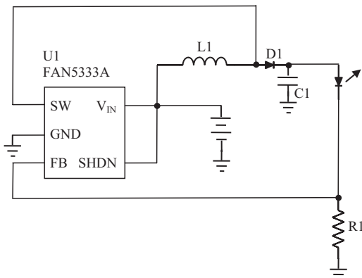
Figure 7.6 FAN5333A Schematic for Boost.
