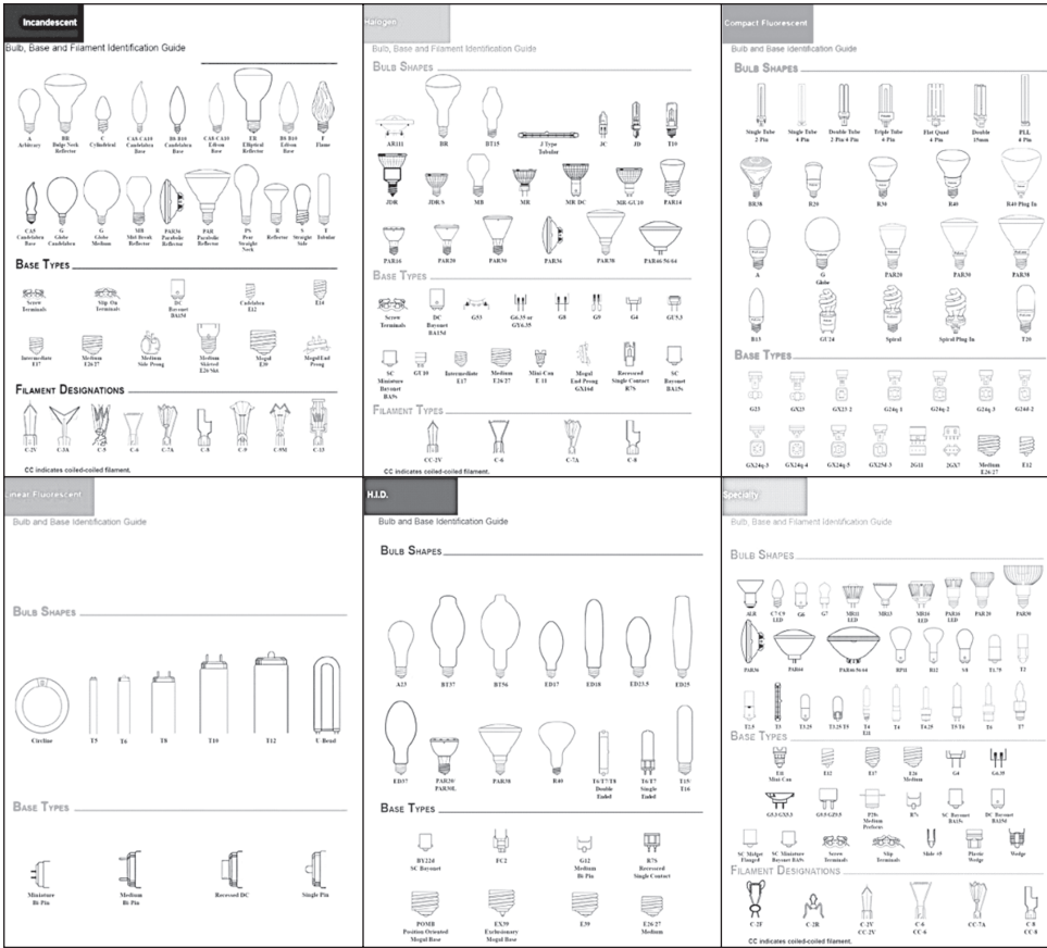
Figure 2.2 Various Bulb Shapes. Illustration courtesy of Halco Lighting Technologies.
