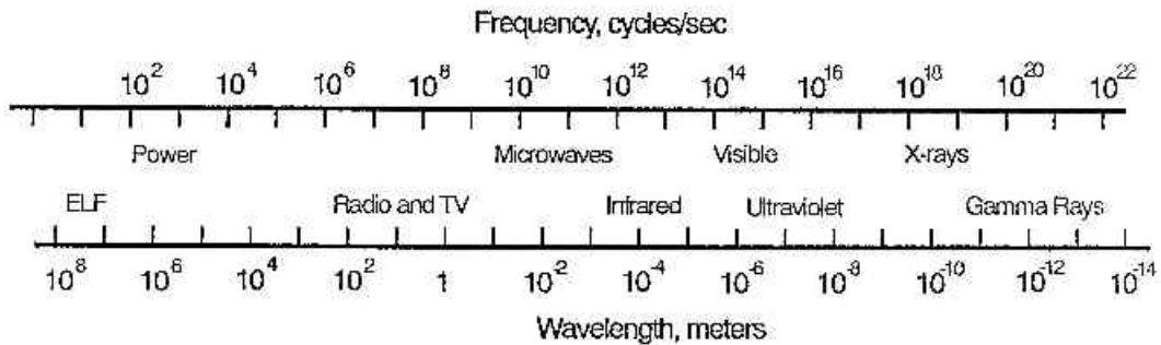
Figure 21-1. Electromagnetic spectrum.
