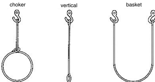
Figure 15-4. Kinds of slings.
