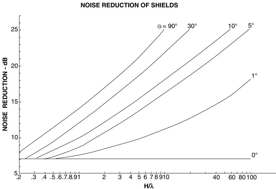
Figure 23-6. Noise reduction for shields. (By permission from The Noise Manual , 5th ed., American Industrial Hygiene Association, Fairfax, VA, 2000.)
