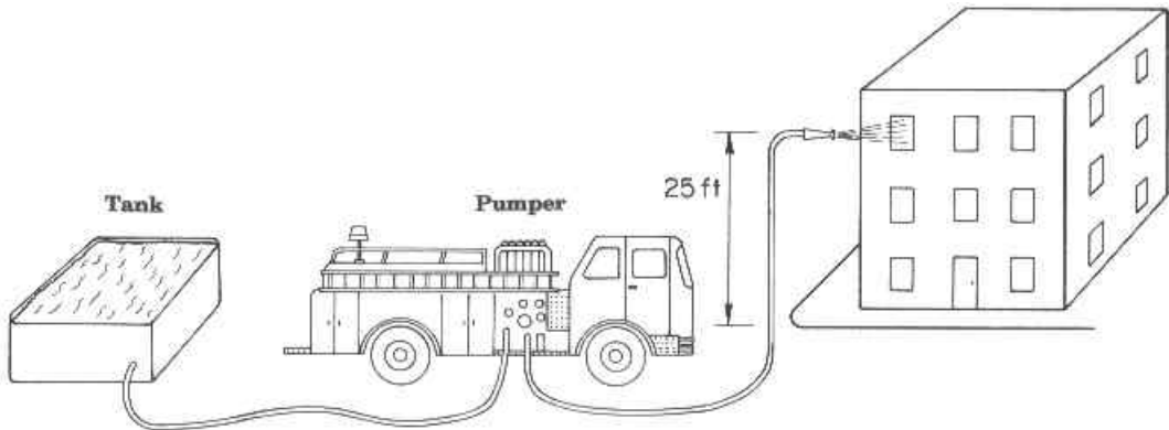
Figure 10-9. Diagram for Example 10-6.
