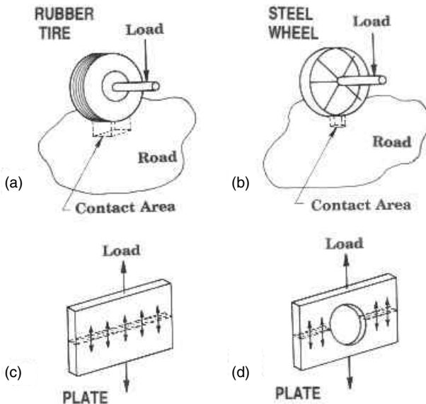
Figure 10-1. Examples of distributed and concentrated forces. In (a) tire flexion distributes the load over a larger road area than does the steel wheel in (b). The hole in the plate in (d) concentrates the load over a smaller internal area compared with the plate without a hole in (c).
