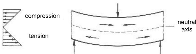
Figure 10-13. Distribution of stress in a beam cross section during bending.
