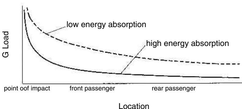
Figure 14-1. Approximate G loads from frontal impact as a function of distance from the point of impact.
