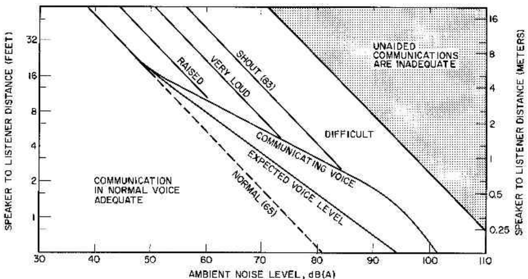
Figure 23-3. Permissible distance between a speaker and listeners for specified voice levels and ambient noise levels. The levels in parentheses refer to voice levels measured 1 m from the mouth. (From MIL-STD-1472D.)
