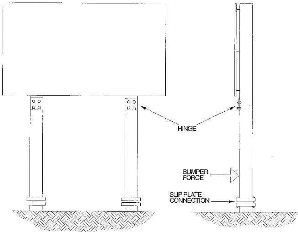
Figure 14-3. Design for break-away highway signs.
