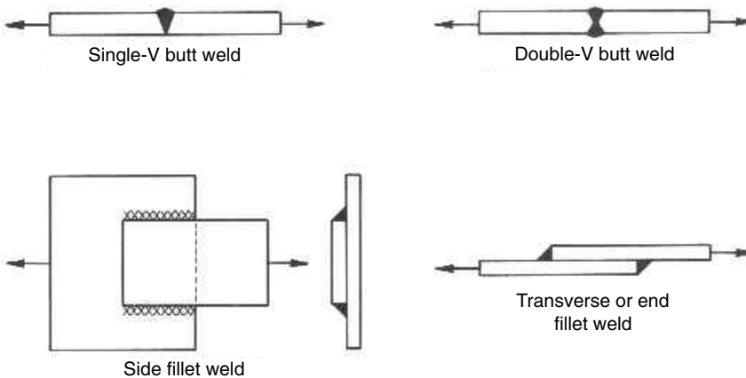
Figure 10-5. Examples of welds.
