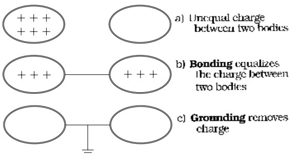
Figure 12-3. Grounding compared with bonding.
