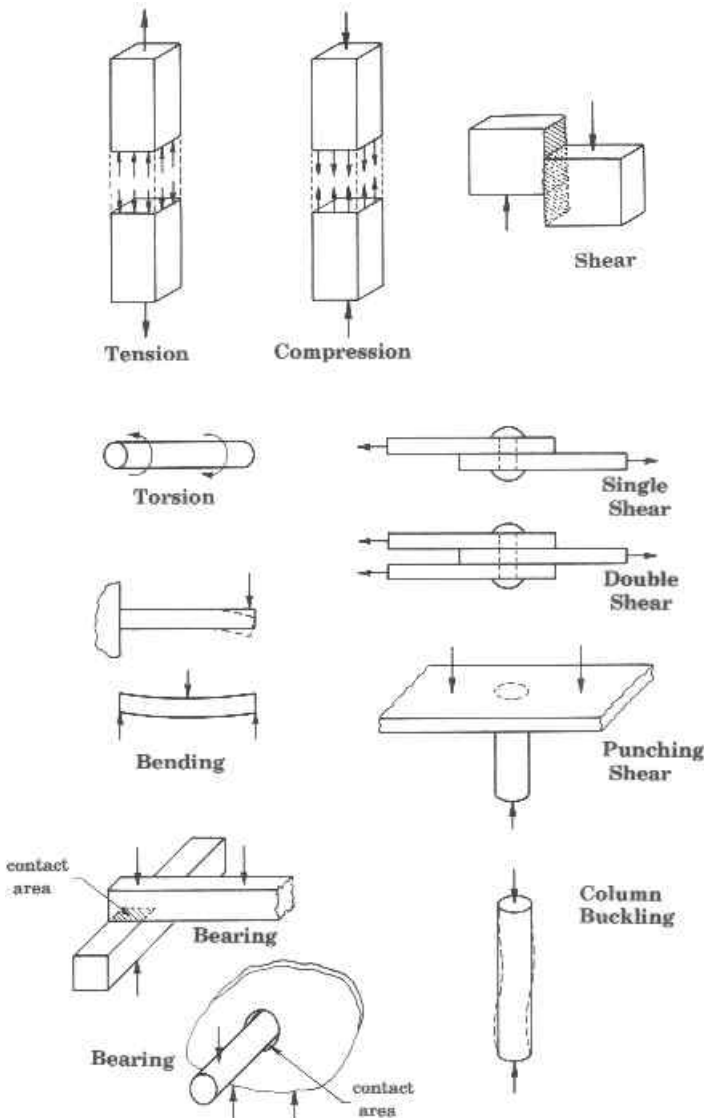
Figure 10-2. Examples of different kinds of stresses and forces.
