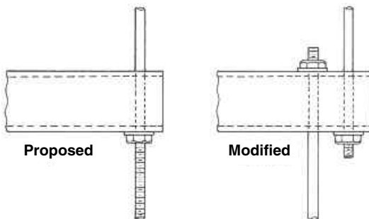
Figure 10-3. Changed load on box beams. In the original design, the load on one skywalk bears on one supporting nut below the box beam. A modification places the load of a lower skywalk on the box beam supporting the upper one. As a result, both loads bear on the nut under the upper box beam.
