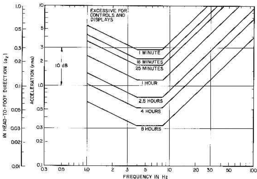
Figure 23-9. ISO standard for whole-body vibration in a vertical direction. The curves give fatigue-decreased proficiency boundaries for vertical (head-to-toe) vibration. For reduced comfort, subtract 10 dB; for safe exposures, add 6 dB. (From MIL-STD-1472D.)
