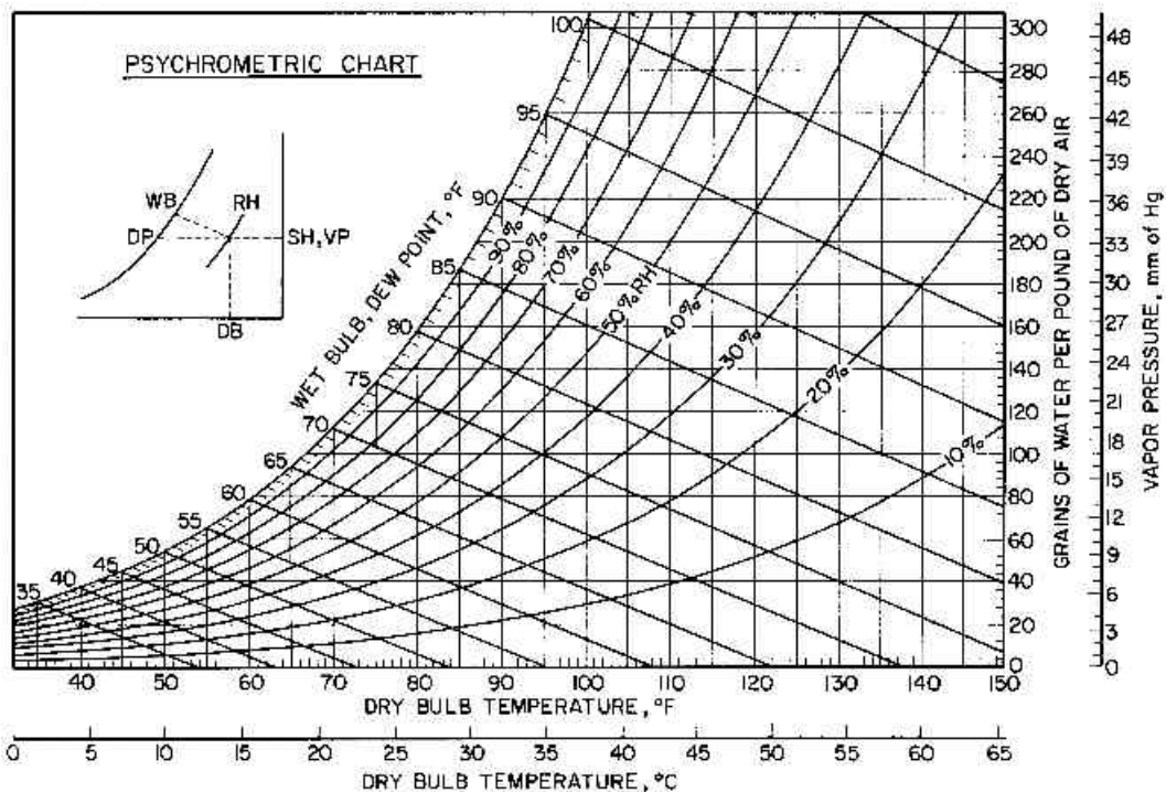
Figure 18-1. Psychrometric chart.
