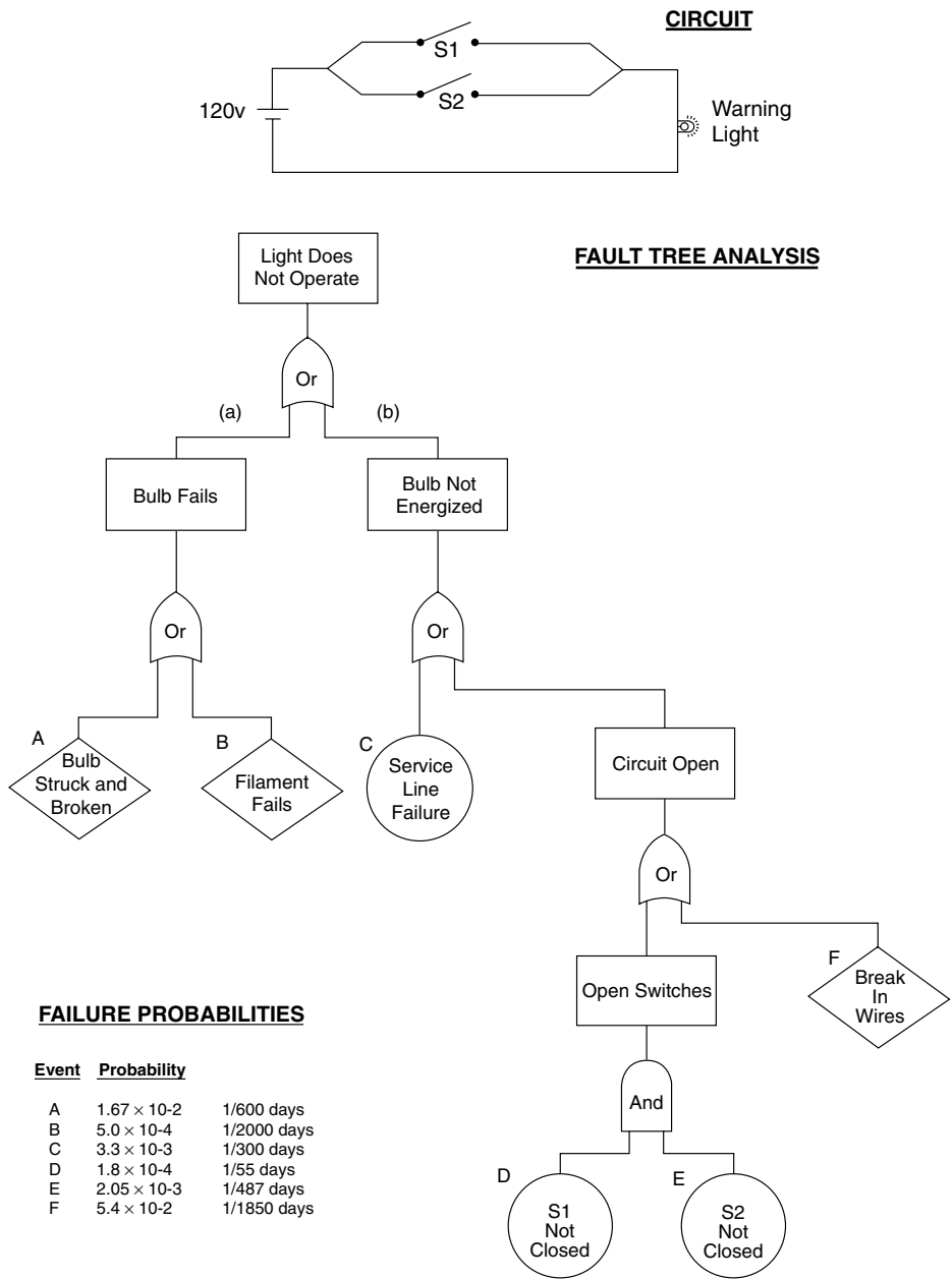
Figure 36-12. System and fault tree diagrams for Exercise 1.
