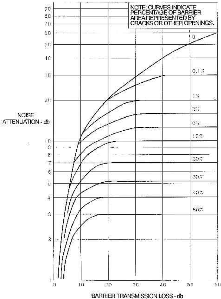
Figure 23-4. Effect of enclosure leaks on barrier sound transmission loss (TL). Enter the chart with the barrier transmission loss for a fully enclosed noise source. Move vertically to intersect with the curve representing the percentage of the barrier area presented by cracks or openings. From the intersection, move left to read the noise attenuation actually achieved.
