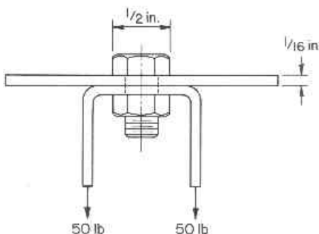
Figure 10-4. Example of tensile strength. The U-shaped member places a tensile load on the bolt.
