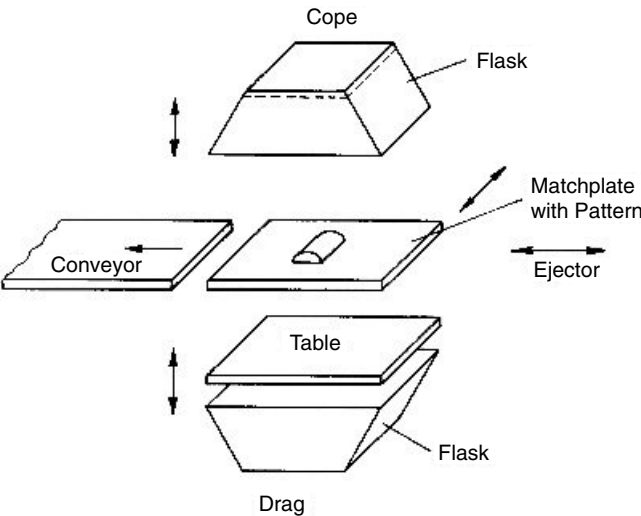
Figure 33-10. Functional diagram of machine components for Exercise 4.
