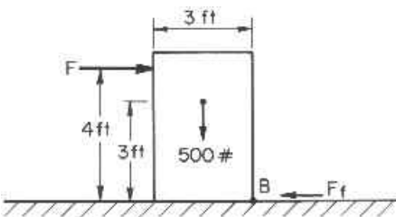
Figure 10-6. Diagram for Example 10-3.
