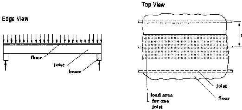
Figure 10-14. Typical structural components and load distribution for a floor.
