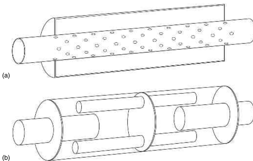
Figure 23-7. Two types of muffler designs. (a) A straight-through dissipative design. (b) A reactive type with baffle and tubes.
