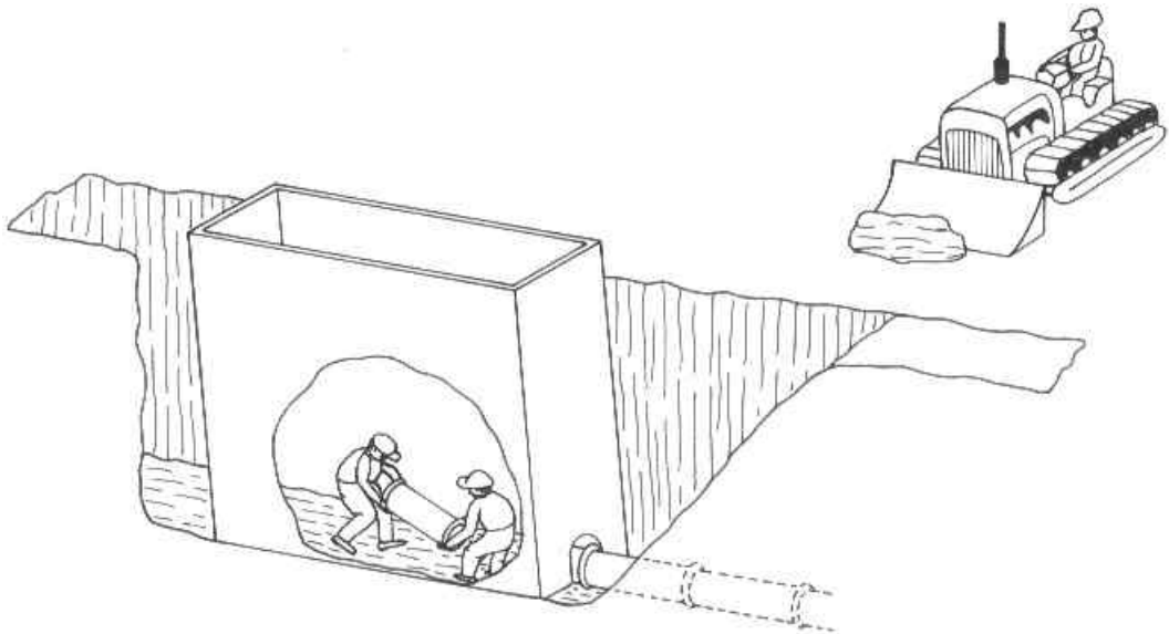
Figure 10-11. A trench shield in use.
