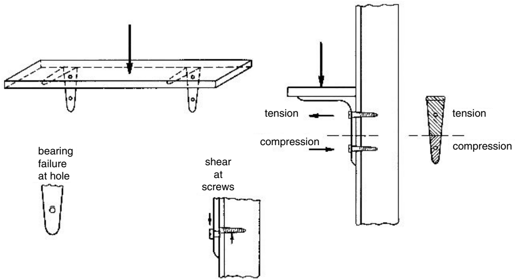
Figure 10-15. A shelf supported by brackets attached to a wall, the load distribution on the brackets, and some modes of failure.
