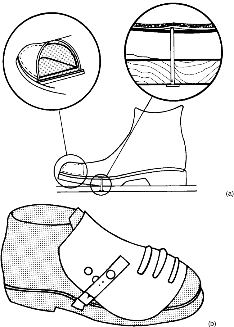
Figure 28-4. Foot protection: (a) exploded view of a safety shoe with safety toe and instep protector; (b) metatarsal guard.
