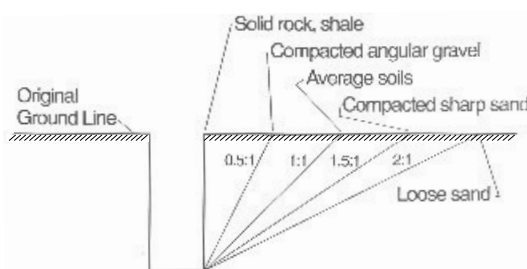
Figure 10-12. Slopes of sides of excavations recommended by OSHA.
