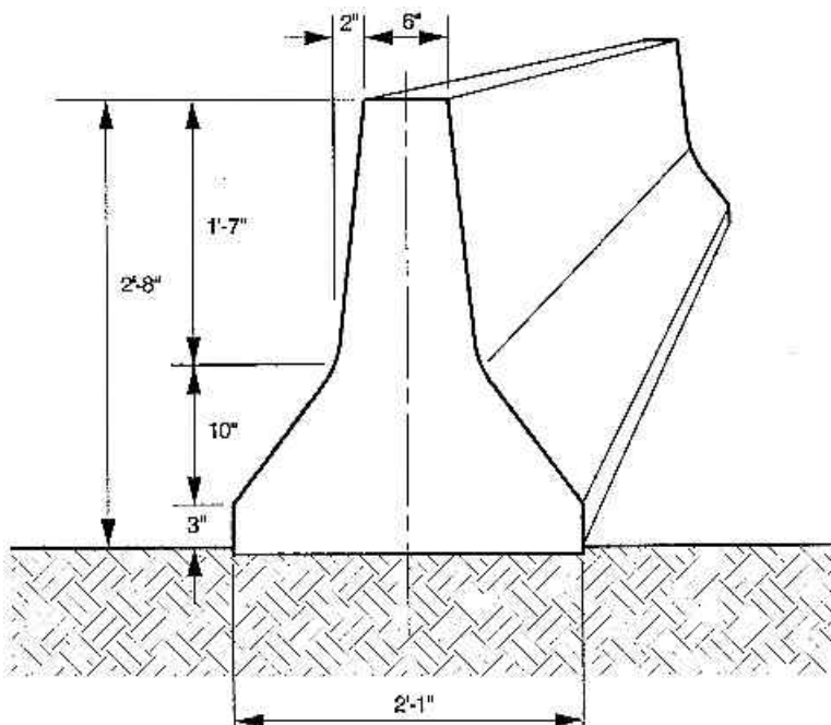
Figure 14-5. Concrete barriers provide protection for highway workers in construction zones, separate opposing traffic lanes and form bridge guardrails.
