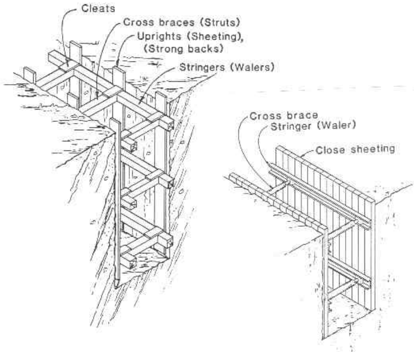
Figure 10-10. Examples of trench shoring and the components involved.
