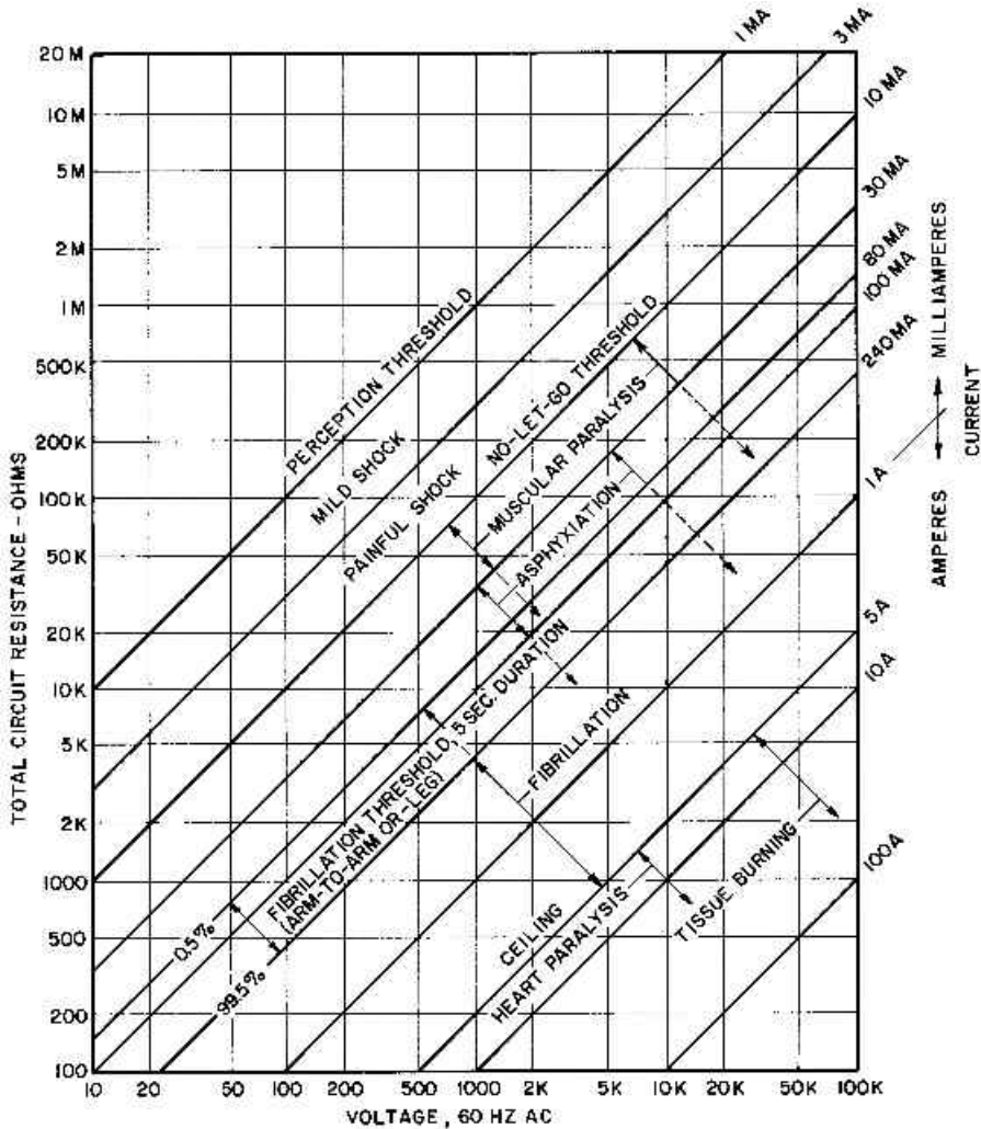
Figure 12-1. Effects of 60 Hz AC electric current on a 150-lb man. (Reprinted by permission. Copyright © by The Instrumentation, Systems and Automation Society, 1965. From Electrical Safety Practices .)
