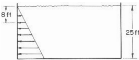
Figure 10-7. Diagram for Example 10-4.
