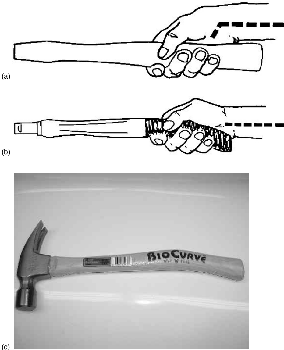
Figure 13-19. Examples of bent handles compared with a straight handle. (a) A conventional hammer handle that requires significant ulnar deviation of the wrist. (b) A curved handle reduces ulnar deviation. (c) A rip hammer with a BioCurve handle. (d) A mallet with a Bio-Curve handle. (Photos of BioCurve tools provided by and used with permission of BARCO Industries Inc., Reading, PA.)
