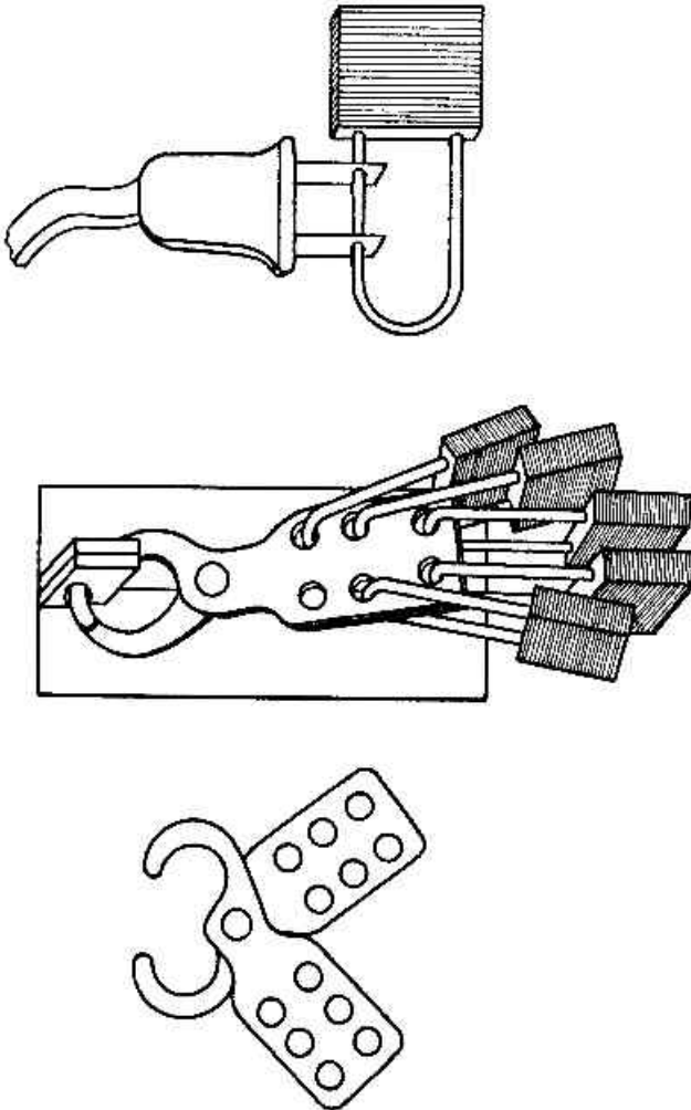
Figure 12-2. Examples of lockout devices.
