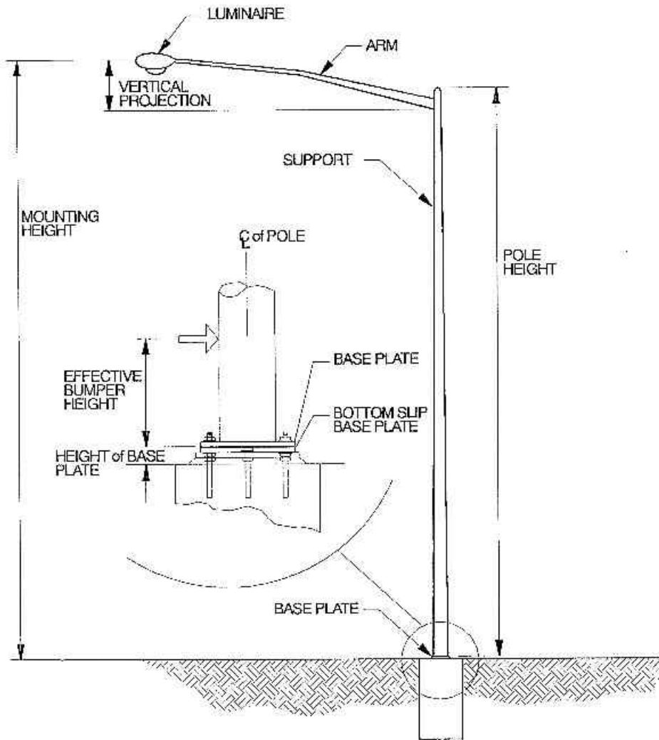
Figure 14-2. Design for break-away light poles.
