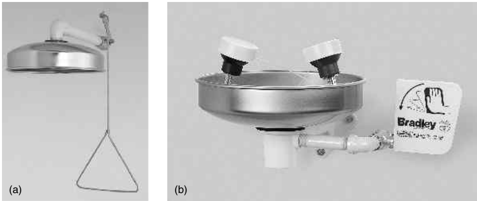
Figure 28-6. Examples of (a) a safety shower and (b) safety eyewash fountain. (Photos provided by and reprinted with permission of the Bradley Corporation, Menomonee Falls, WI.)
