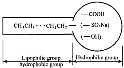
Figure 5.4 The Composition Diagram of Surfactant Molecules
