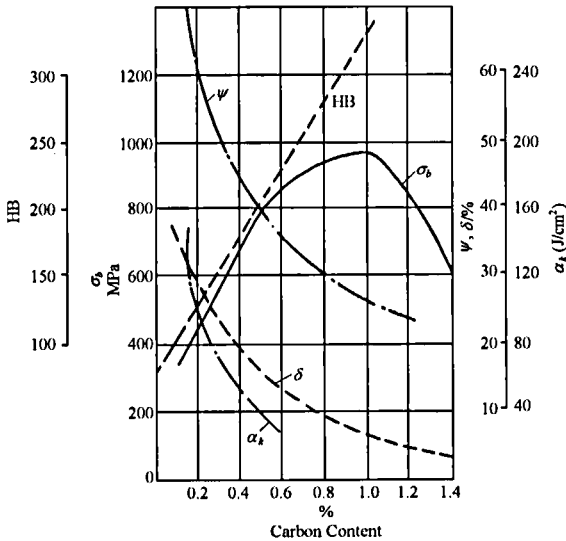
Figure 8.7 Influences of Carbon Content on Properties of Hot-rolled Carbon Steel \sigma_b . Tensile Strength ; \alpha_k .Impact Toughness; HB. Hardness; \delta .Elongation; \phi . Shrinkage of Cross-section
