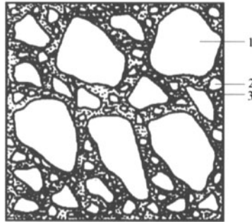
Figure 5.1 The Ordinary Cement Structure
