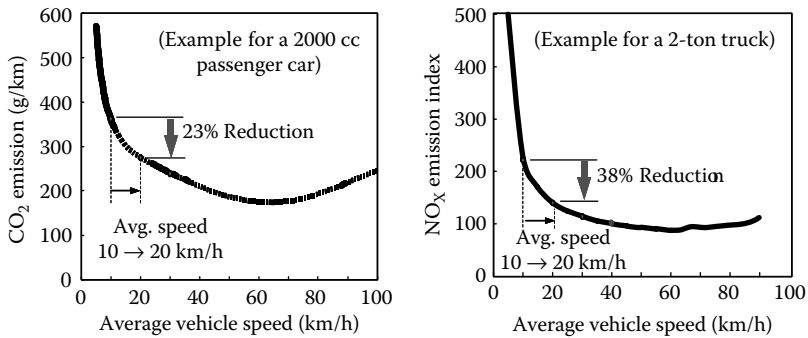
FIGURE 1.6 Emission levels as a function of average vehicle speed. 4
