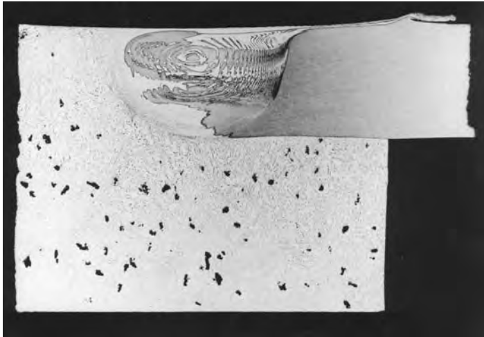
FIGURE 15.5 Wrought aluminum welded to cast aluminum alloy.
