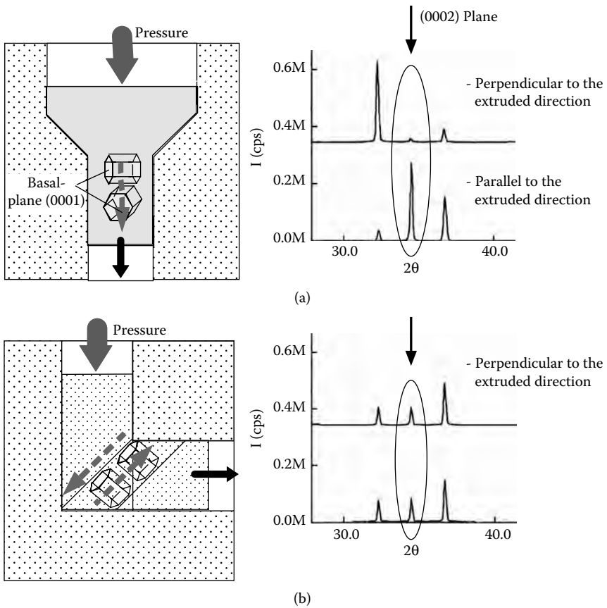
FIGURE 10.4 Schematic illustration and X-ray diffraction spectra of (a) the directly extruded AZ31 alloy and (b) AZ31-E/A.
