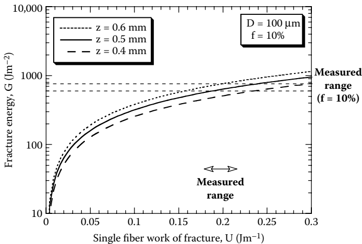
FIGURE 14.13 Predicted dependence (Equation 14.26) of the interlaminar fracture energy of the 3-D fiber array on the single fiber work of fracture.
