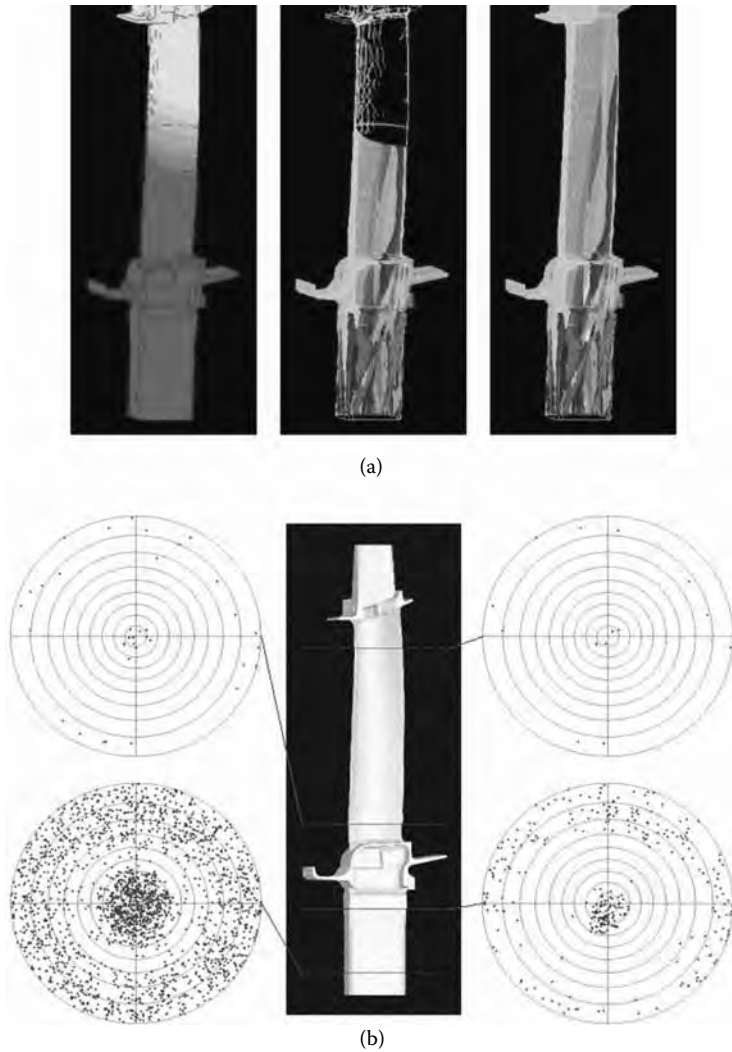
FIGURE 17.10 Prediction of grain structure (a) and orientation with pole figure (b) in a directionally cast turbine blade.
