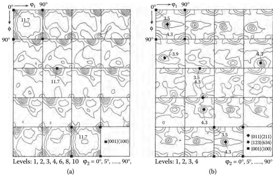
FIGURE 9.1 Orientation distribution functions of (a) 5052 and (b) 6061 aluminum alloy sheets cold rolled to 90% reduction and subsequently annealed for 3 ks at 573 and 623 K, respectively.
