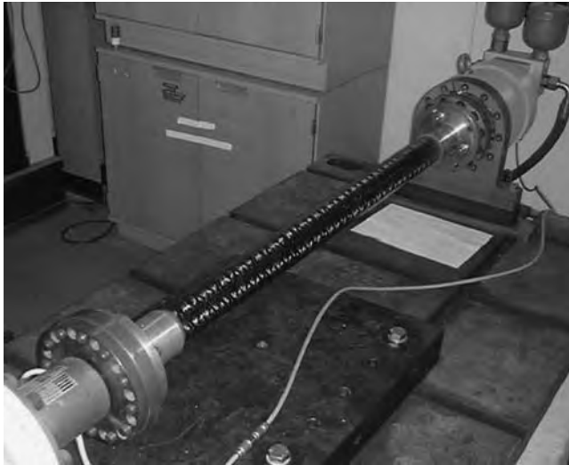
FIGURE 19.3B Testing of assembled CFRP prop-shaft.
