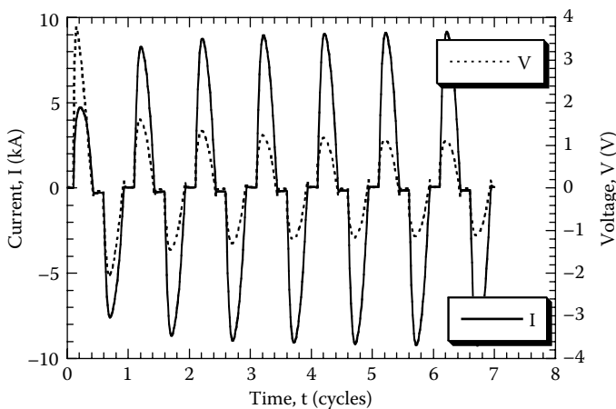
FIGURE 14.17 Voltage-time and current-time plots obtained during welding together of two brazed in-plane mesh sheets, with a weld time of 7 cycles (0.14 s).
