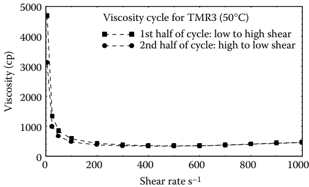
FIGURE 5.4a Viscosity versus shear rate for a typical magnetorheological fluid in zero-applied field.
