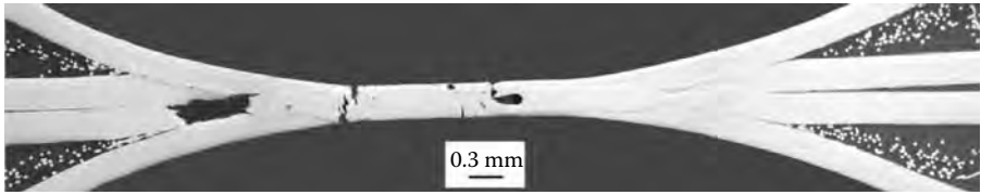
FIGURE 14.16 Optical micrograph of a polished transverse section from a pair of flocked sheets after resistance welding.
