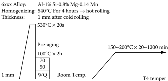
FIGURE 2.3 Study of the bake-hardening properties of 6xxx alloys after pre-aging.
