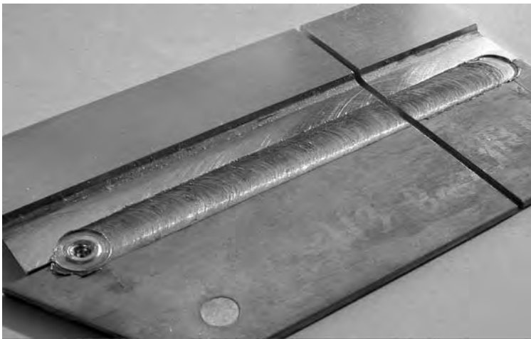
FIGURE 15.6 Friction stir weld between aluminum and magnesium alloys.
