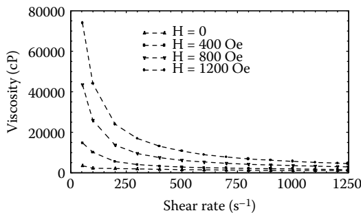
FIGURE 5.4b The effect of applied DC magnetic field on the viscosity of a typical magnetorheological fluid.
