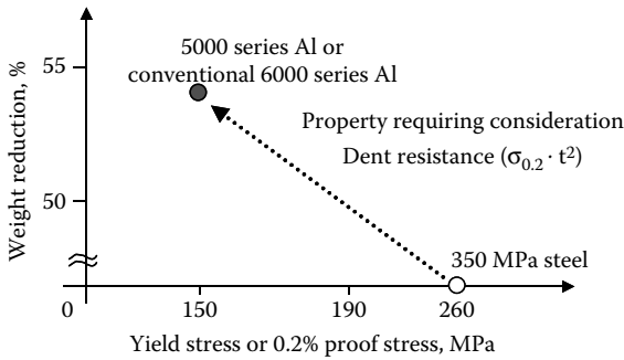
FIGURE 1.11 Reduction of outer panel weight by substituting aluminum for steel sheet.
