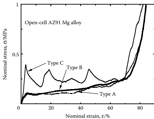
FIGURE 12.7 The nominal stress–nominal strain curves of the cellular Mg.
