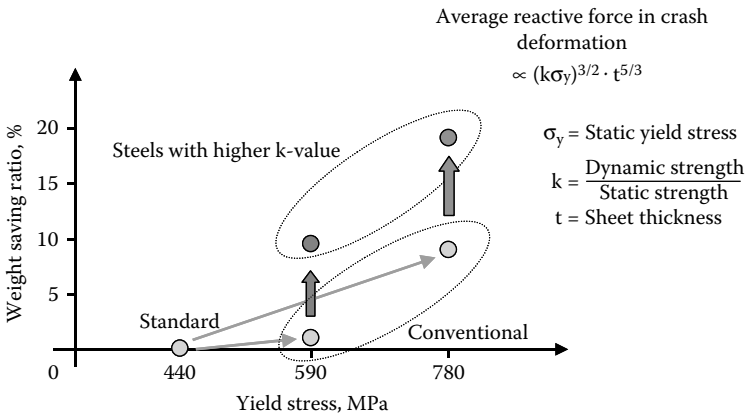
FIGURE 1.15 Part weight reductions achieved by using high-strength steel with a higher k-value.
