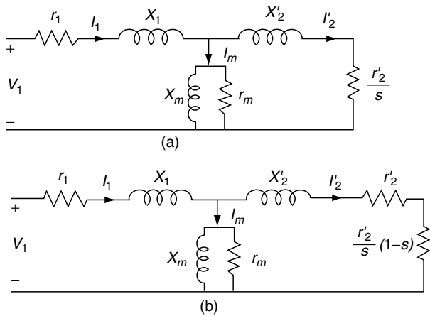
FIGURE 4.17 Phase-Equivalent Circuit of Polyphase Induction Motor
