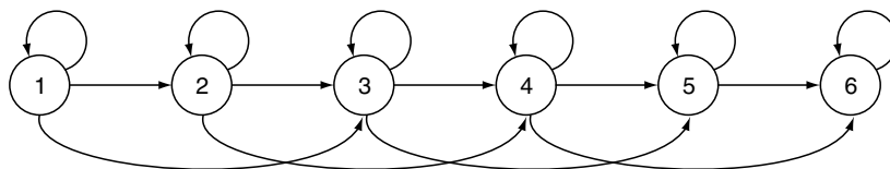
FIGURE 3.11 Typical HMM with Six States
