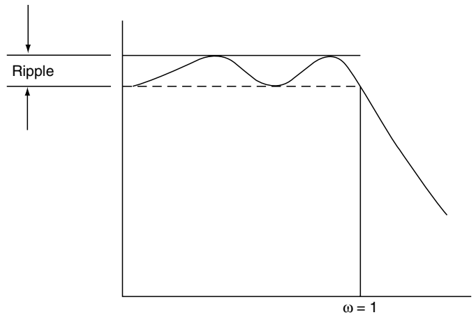
FIGURE 4.18 Amplitude Response of a Chebyshev Filter
