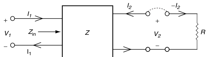
FIGURE 4.6 Obtaining Input Impedance of a Two Port Loaded by a Resistor
