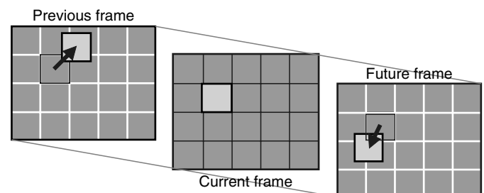
FIGURE 6.5 Motion Estimation in B-Pictures
