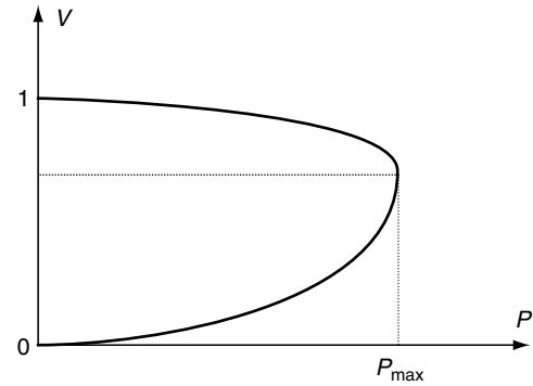
FIGURE 7.10 Qualitative Plot of the Power-Flow Solutions
