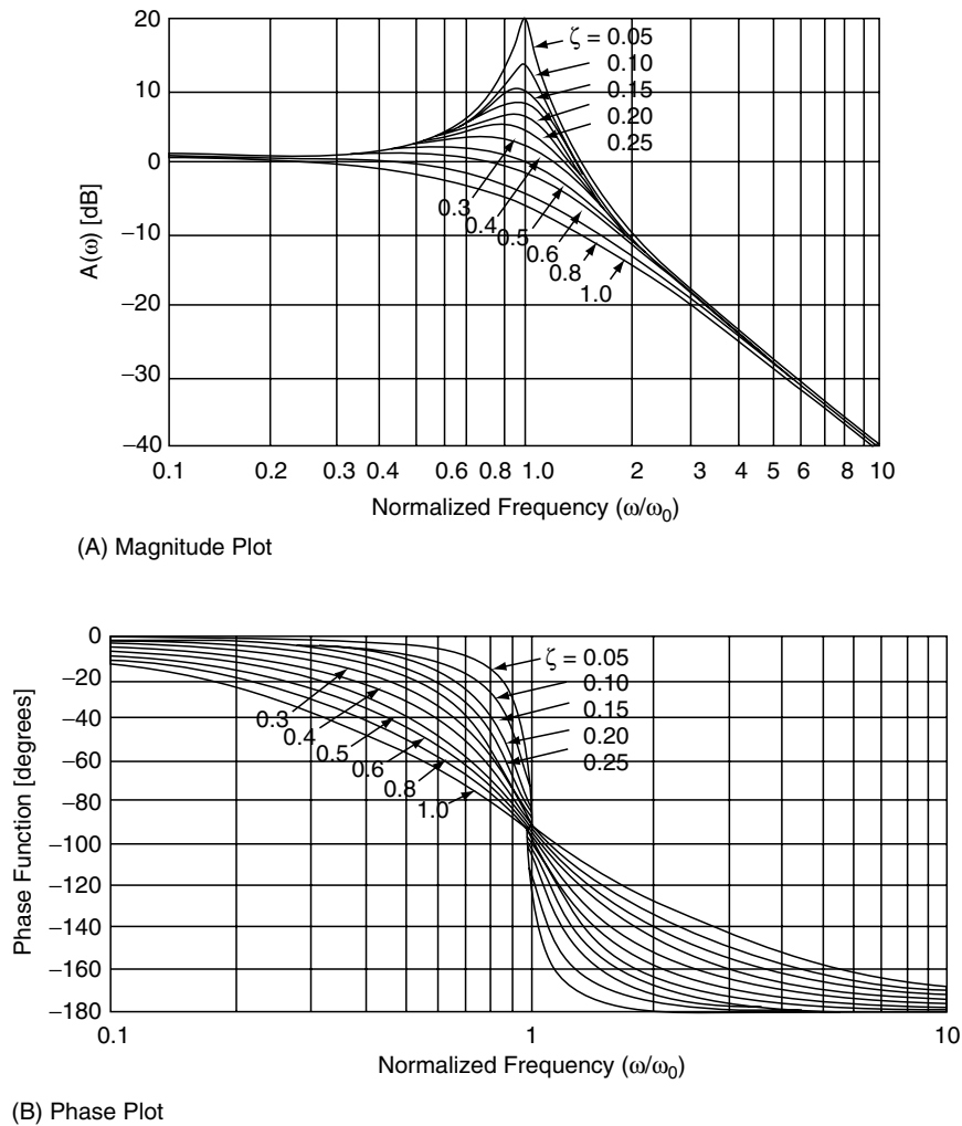
FIGURE 1.32 Bode Diagrams of H(j\omega) = [(\omega_0^2 - \omega^2) + j(2\zeta\omega_0\omega)]^{-1}
