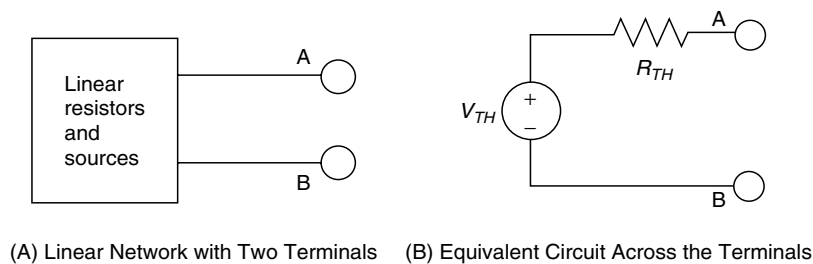
FIGURE 1.15 Thevenin Equivalent Circuit
