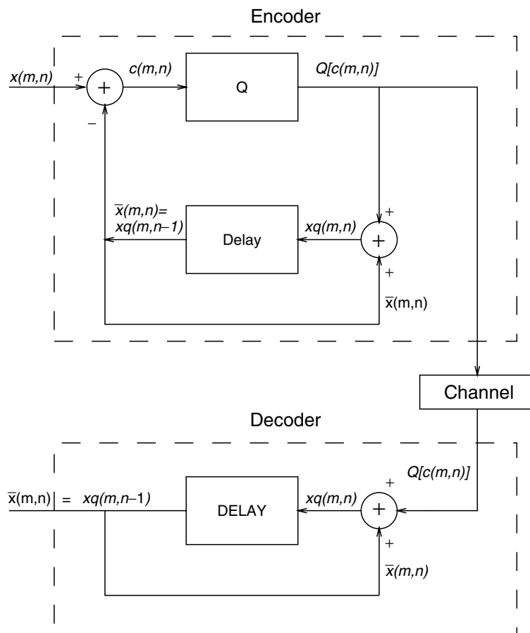
FIGURE 4.19 DPCM Encoder/Decoder
