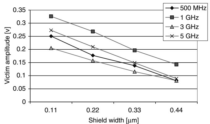
FIGURE 8.9 Noise Amplitude Versus Shield Width at Different Frequencies
