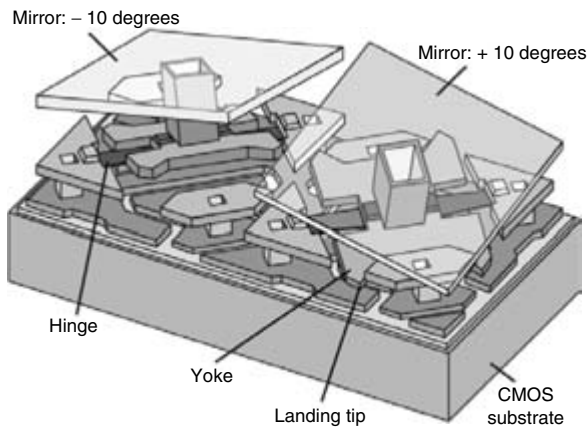
FIGURE 6.13 Drawing of Two Pixels of the Digital Mirror Device Manufactured by Texas Instruments. The torsional hinges are 5 by 1\text{ }\mu\text{m} in area and about 100 nm thick. The individual mirrors are 16\text{ }\mu\text{m} square. Over 500,000 of them are found in a single device, making this the system with the most moving parts produced in the history of mankind. The inventor, Larry Hornbeck, and the company received television Emmy Awards in 1998 for outstanding achievement in engineering development. Figure provided by Hornbeck (1993).
