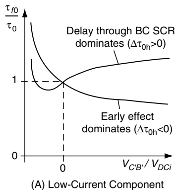
FIGURE 5.8 Bias Dependence of the Forward Transit Time. (A) This graph shows the low-current component for different cases ( V_{C'B'} = V_{CB} ). (B) Notice the current dependence shown here; high-current effects start for I_C > I_{CK} . Typical units: \tau_f in ps; \bar{Q}_f in fC/ \mu\text{m}^2 .
