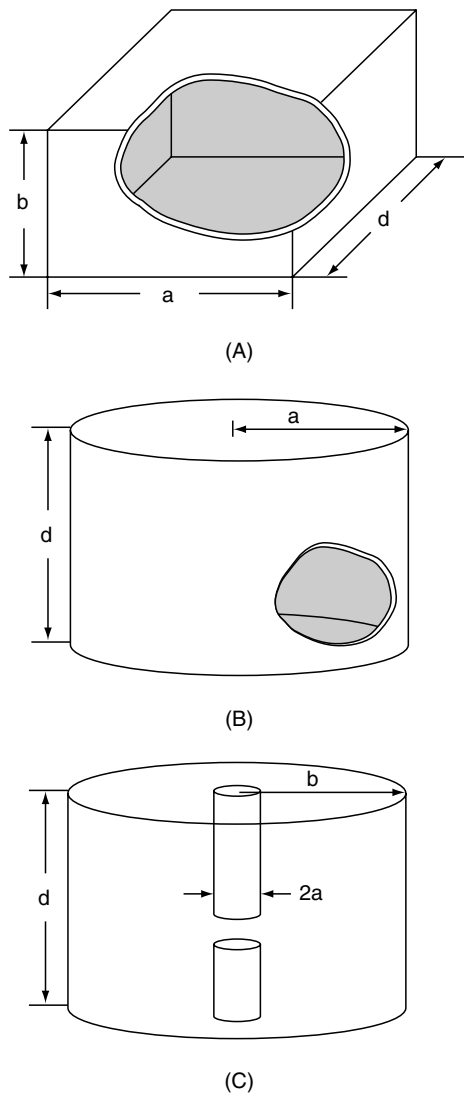
FIGURE 7.26 Representative Waveguide and Coaxial Line Cavity Resonators
