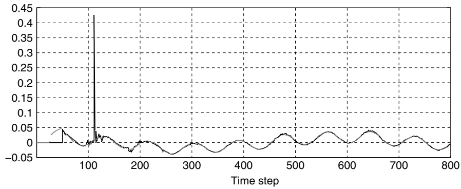
FIGURE 8.10 Output Prediction, nfy2 , from the Online Estimator Versus Actual Failure Dynamics Output, fy2 (MIMO System; 25-Data Window). Solid line: Output ( nfy2 ) of online estimator/Dashed line: Actual failure output ( fy2 ).
