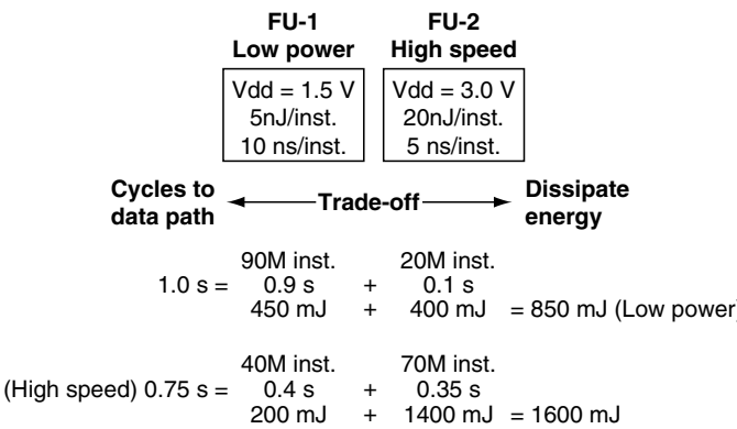
FIGURE 2.18 Data Path Example of a Performance Versus Energy Trade-Off
