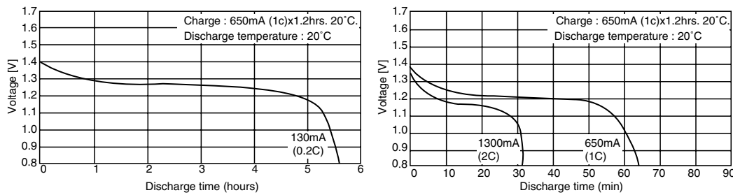
FIGURE 5.14 Indicates that the Battery Life Depends on the Amount of Average Current Discharged, Noting that the Charging Process was Identical in the Three Cases and More Current Means More Power Withdrawn; the figure shows three different average discharge currents values: 130 mA, 650 mA, and 1300 mA. The 130 mA average discharge current gave the longest discharge time of all three and the 1300 mA average discharge current gave the shortest time.
