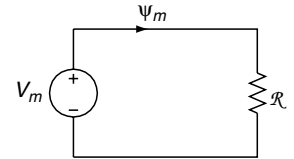
(B) Equivalent Magnetic Circuit
