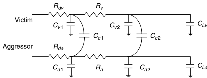
FIGURE 8.6 Interconnect Distributed \pi Model (for the Configuration in Figure 8.4)
