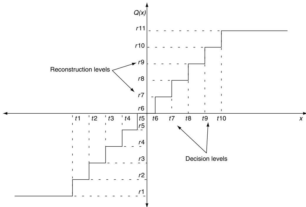
FIGURE 4.9 Typical Quantizer
