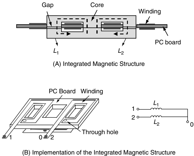
FIGURE 1.21 Integrated Magnetic Structure
