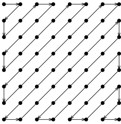
FIGURE 4.23 Scanning Order of the Quantized DCT Coefficients
