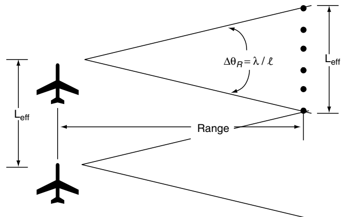
FIGURE 10.7 A Side-Looking SAR Geometry
