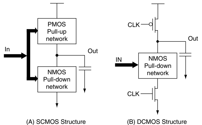
FIGURE 5.20 (A) SCMOS general structure has two complementary networks: PMOS pull-up network for charging the output into V_{dd} , and NMOS pull-down network to discharge the output to GND . The SCMOS style requires 2N transistors to implement a function. (B) DCMOS general structure has only an NMOS pull-down structure. The DCMOS style operates in two phases controlled by a clocking signal, CLK . When CLK = 0 , the DCMOS gate is in the precharge state, where the PMOS transistor controlled by CLK is on allowing the output to charge to V_{dd} . At the same time, the pull-down network is off since the NMOS transistor controlled also by CLK is off ( CLK = 0 ). When CLK = 1 , the evaluate state takes place, allowing the output to be evaluated as a function of the input. DCMOS style requires N + 2 transistors to implement a function.
