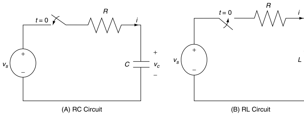
FIGURE 1.20 Circuits with a Single Energy-Storing Element
