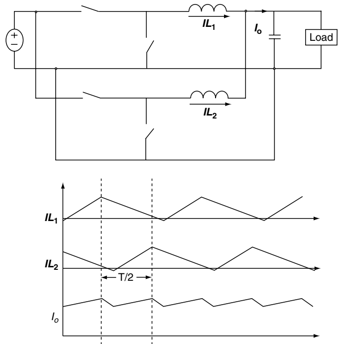
FIGURE 1.16 Current Ripple Cancelling Effect of Interleaved QSW
