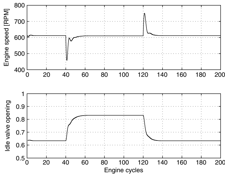
FIGURE 10.8 Engine Speed Variations and Control Input (Simulation)
