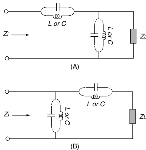
FIGURE 7.14 Generalized Lumped-Element Network Transformers with Various L-C Combinations
