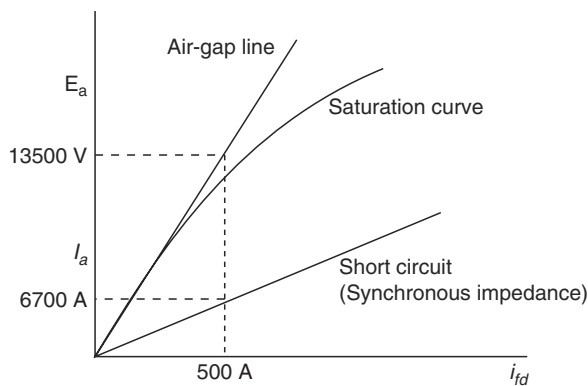
FIGURE 4.26 Open Circuit Test
