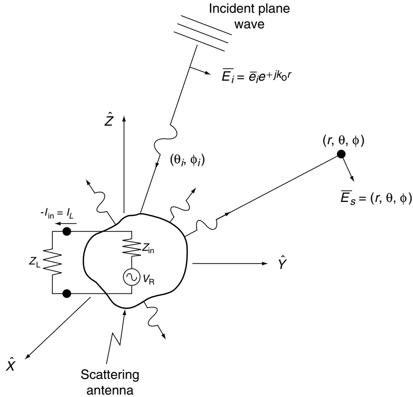
FIGURE 6.9 A Plane Wave Incident From Angle (\theta_i, \phi_i) is Scattered from an Antenna. The scattered signal \vec{E}_s(r, \theta, \phi) is observed at a point (r, \theta, \phi) . The scattered signal is affected by the load impedance Z_L .
