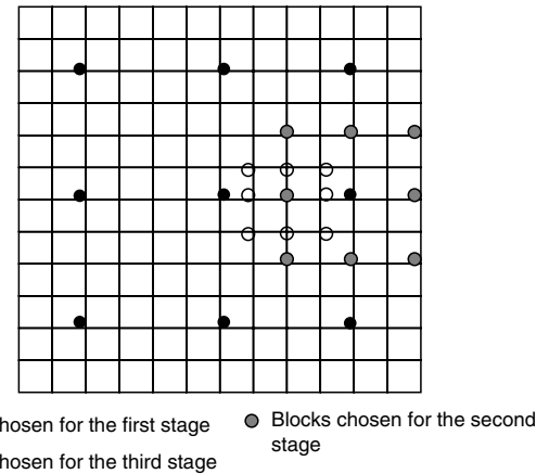
FIGURE 6.3 Example Path for Convergence of a Three-Step Search
