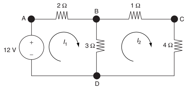
FIGURE 1.4 Circuit for Example 1.2
