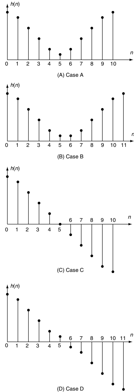
FIGURE 2.7 Linear-Phase FIR Filter: Typical Impulse Response
