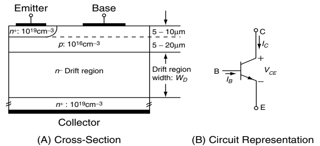
FIGURE 7.4 Power Bipolar Junction Transistor
