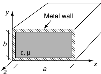
FIGURE 5.5 Cross Section of Dielectric-Filled Metallic Rectangular Waveguide
