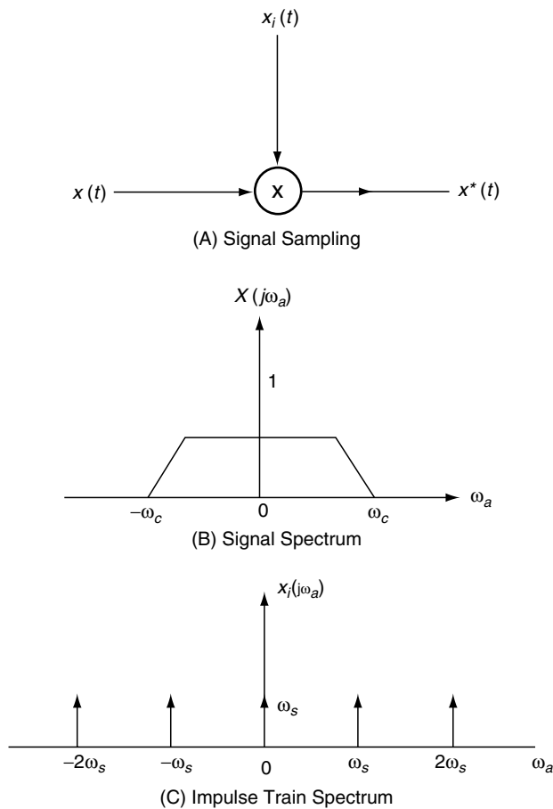
FIGURE 2.2 Sampling of Continuous-Time Signals
