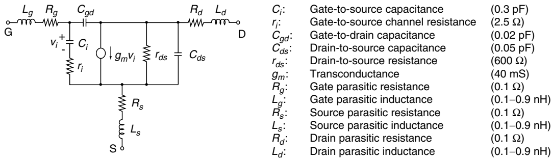
FIGURE 11.6 Equivalent Common-Source Model of Typical MOSFET. This model includes packaging effects.
