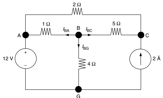
FIGURE 1.9 Circuit for Example 1.5
