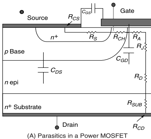
FIGURE 7.12 MOSFET Device
