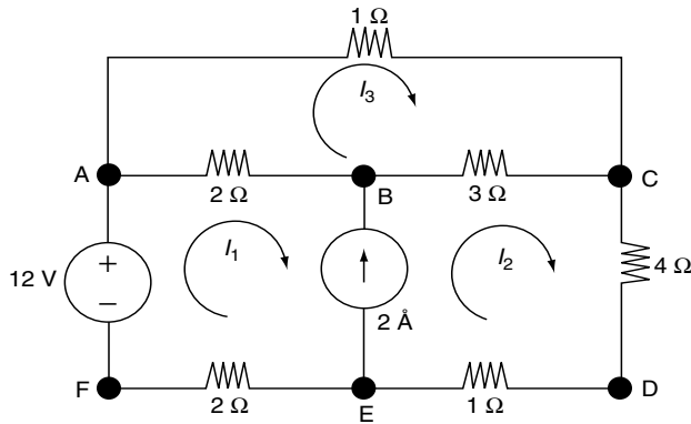
FIGURE 1.6 Circuit for Example 1.4
