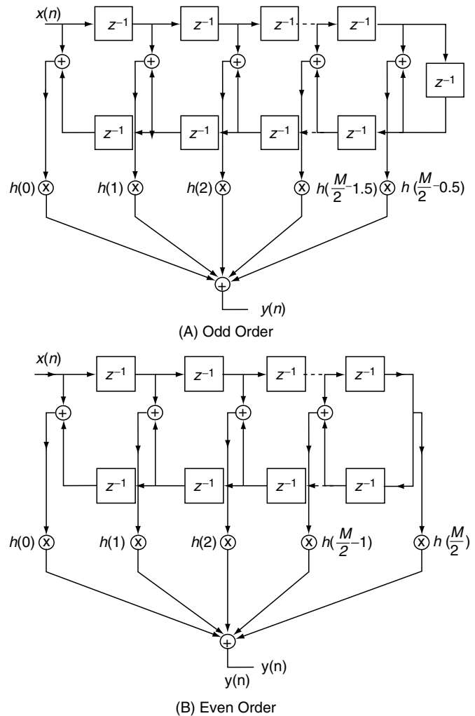
FIGURE 2.10 Linear-Phase FIR Filter Realization With Symmetric Impulse Response
