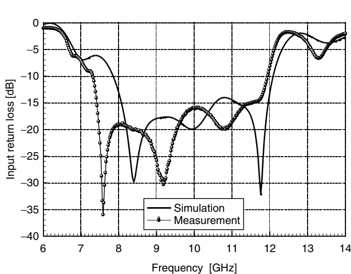
FIGURE 11.21 Input Return Loss (Left) and Measured Radiation Characteristics (Right) of X-Band Quasi-Yagi Antenna
