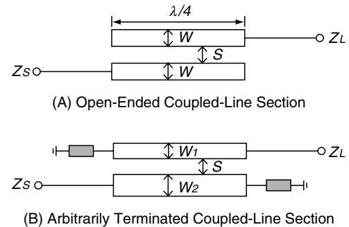
FIGURE 7.13 Two Representative Quarter-Wavelength Coupled-Line Sections for Impedance Transformation and Matching Purposes
