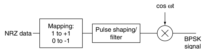
FIGURE 4.2 BPSK Modulator
