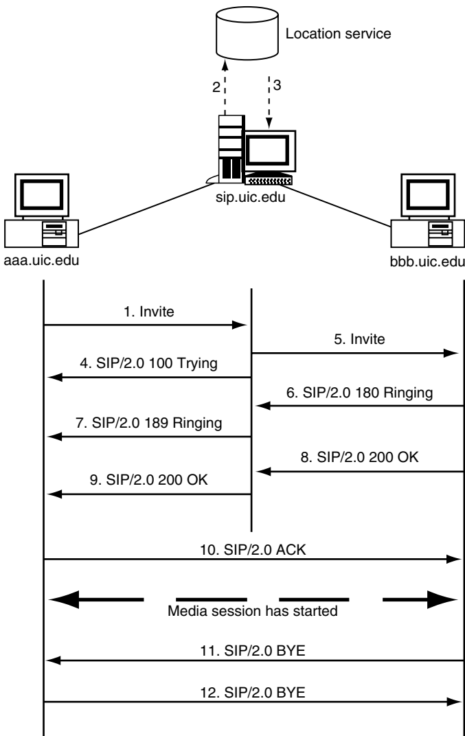
FIGURE 7.11 Timeline for a Typical SIP Session
