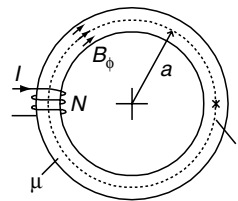
(A) Physical Geometry
