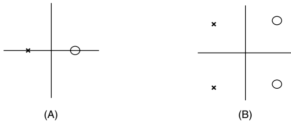
FIGURE 4.32 Possible Pole-Zero Positions for All-Pass Networks
