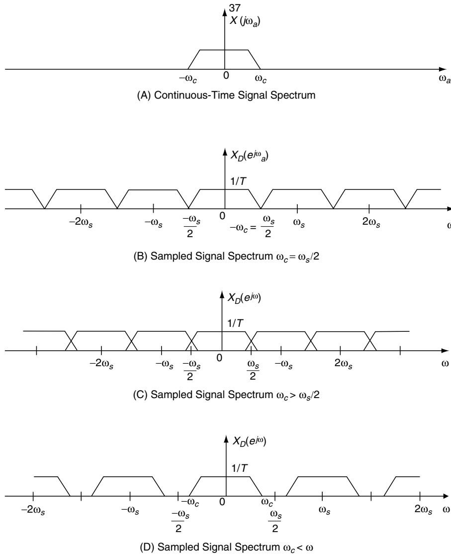
FIGURE 2.4 Sampling Effects
