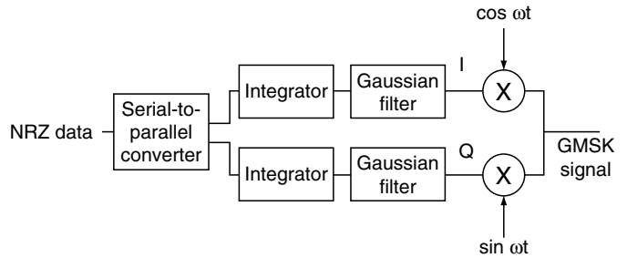
FIGURE 4.13 GMSK Modulator Using Phase Modulator
