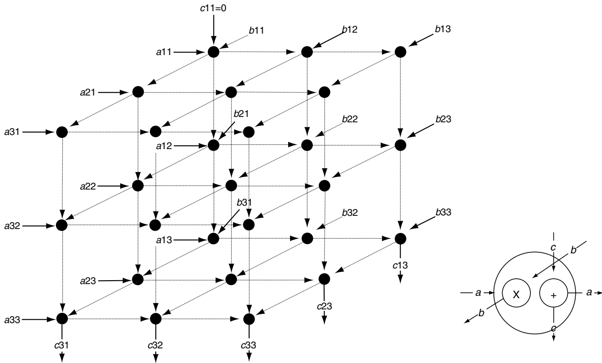
(A) A 3 x 3 Matrix-Matrix Multiplication in a 3-D Dependence Graph
