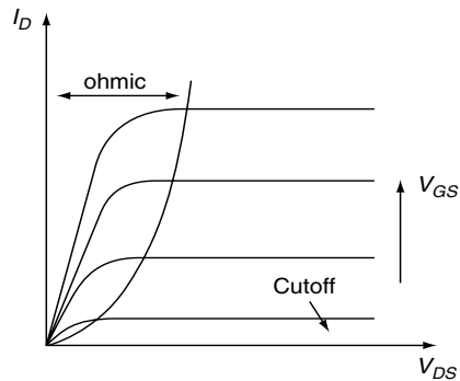
(B) Typical Output Characteristics
