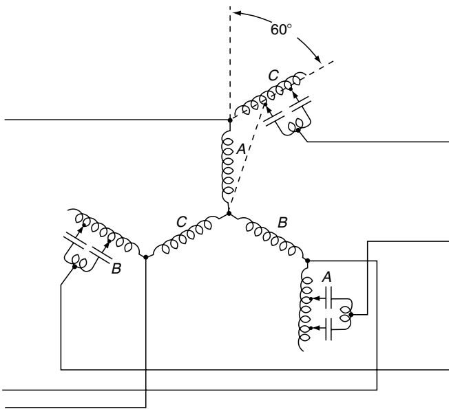
FIGURE 3.4 Phase-Angle Regulator
