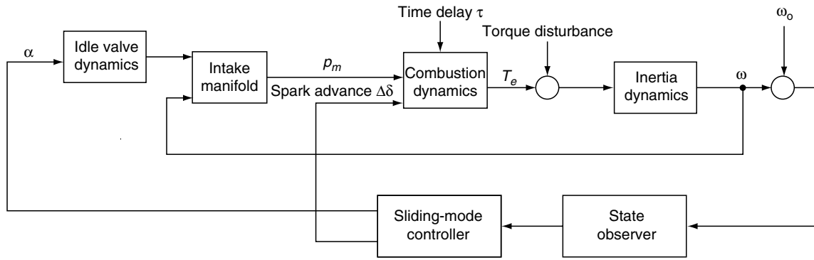
FIGURE 10.1 Point-Delayed SMC Structure
