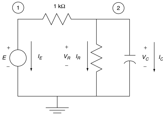
FIGURE 3.5 Nonlinear Circuit
