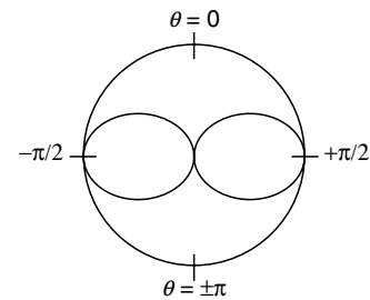
(B) Power Radiation Pattern
