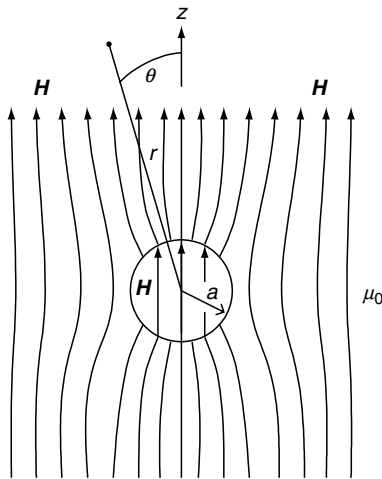
FIGURE 1.5 Magnetic Sphere of Permeability \mu Immersed in a Uniform \mathbf{H} Field. The field lines become strictly vertical when the sphere is removed.
