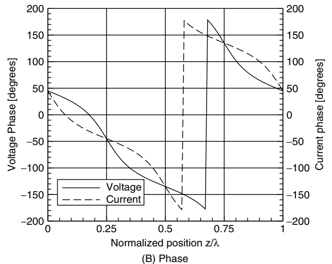
FIGURE 4.10 Voltage and Current on a Resistively Terminated Lossless Line
