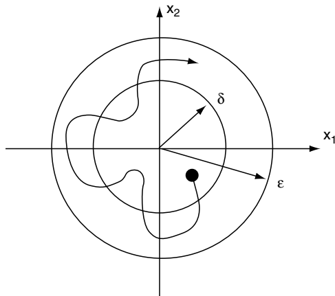
FIGURE 2.8 Typical Behavior of the Trajectory in the Vicinity of a Stable Equilibrium. This is true whenever x(0) \leq \delta(\varepsilon) .
