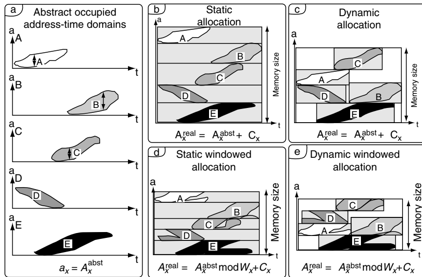
FIGURE 2.27 Intrasingal and Intersignal In-Place Data Mapping
