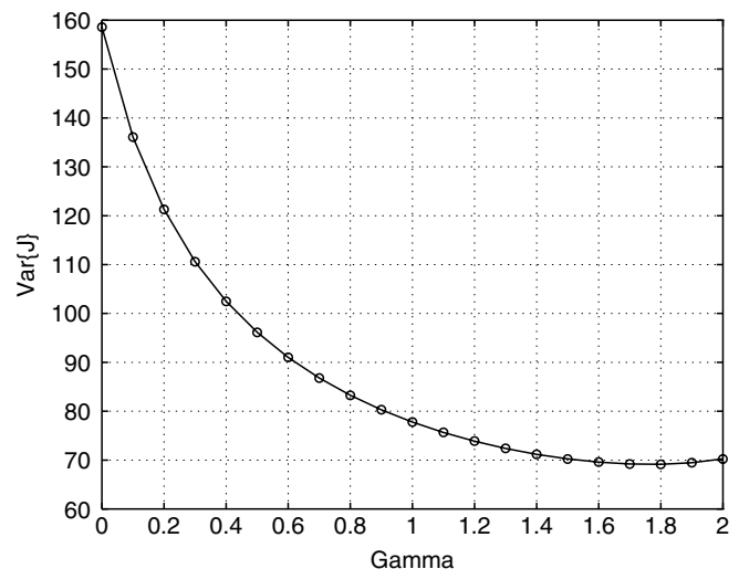
FIGURE 5.5 Optimal Variance: Full-State Feedback, MCV, 3DOF
