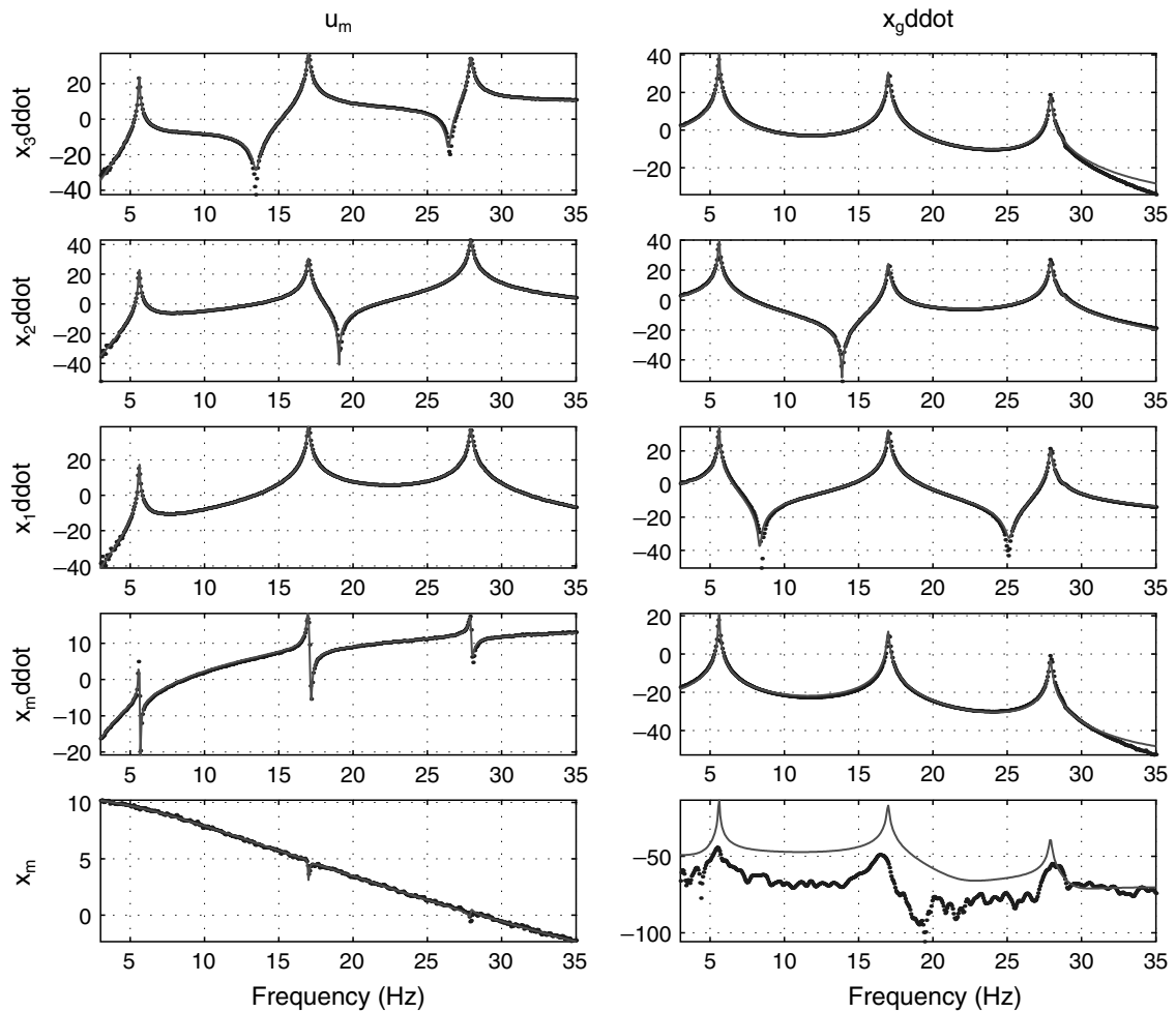
FIGURE 6.6 Comparison of Experimental and Model FRF for the Seismic-AMD Benchmark Structure: Magnitude Plot. u_m denotes the input command to the AMD; x_g\ddot{\cdot} denotes the input ground acceleration to the structure; x_j\ddot{\cdot} denotes the output acceleration of the j th floor; x_m\ddot{\cdot} denotes the output acceleration of the AMD; x_m denotes the output displacement of the AMD; dotted lines are for measurement data; solid lines are for model output.
