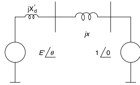
FIGURE 7.14 A Simple Power System
