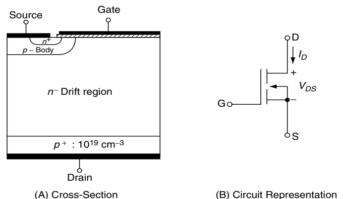
FIGURE 7.11 Power MOSFET
