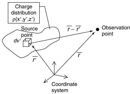
FIGURE 2.3 Definition of the Prime and Unprimed Coordinates for Source-Field Relationships
