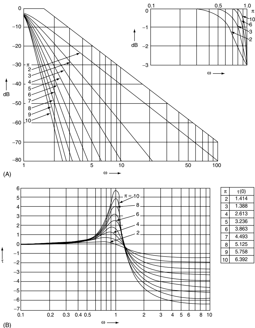
FIGURE 4.16 (A) Selectivity Curves of Maximally Flat Filters (B) Group Delay of Maximally Flat Filters
