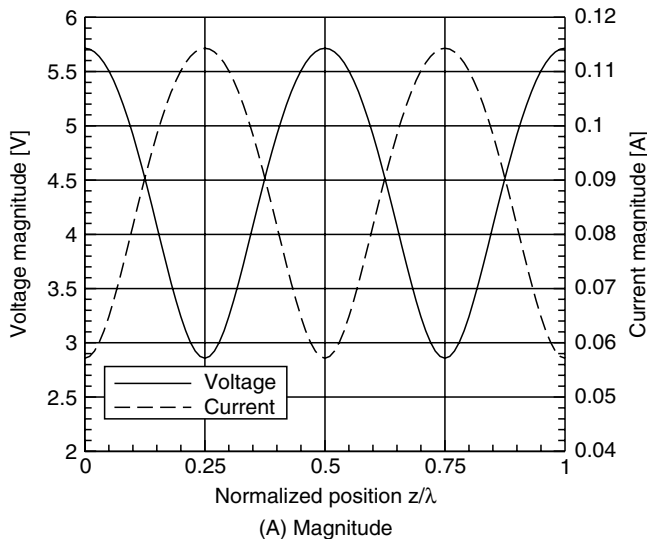
FIGURE 4.10 Voltage and Current on a Resistively Terminated Lossless Line
