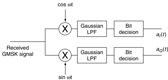
FIGURE 4.14 GMSK Demodulator
