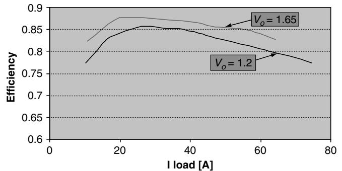
FIGURE 1.34 Push-Pull Forward Efficiency (A) Efficiency of the Push-Pull Forward Converter ( V_{in} = 48 V, V_o = 1.2 V, f_s = 100 kHz; secondary side uses four MTP75N03DHL, and primary side uses two IRL3103D1). (B) Efficiency of the Push-Pull Forward Converter ( V_{in} = 12 V, f_s = 100 kHz; secondary side uses four MTP75N03DHL, and primary side uses two IRL3103D1).
