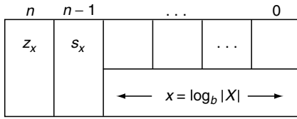
FIGURE 1.1 The Organization of an (n + 1) -bit LNS Digital Word
