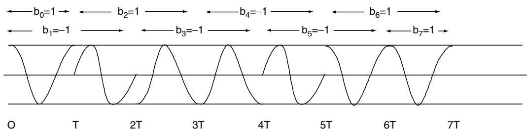
FIGURE 4.7 OQPSK Signals
