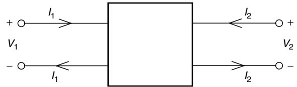
FIGURE 4.3 Symbol for a Two-Port
