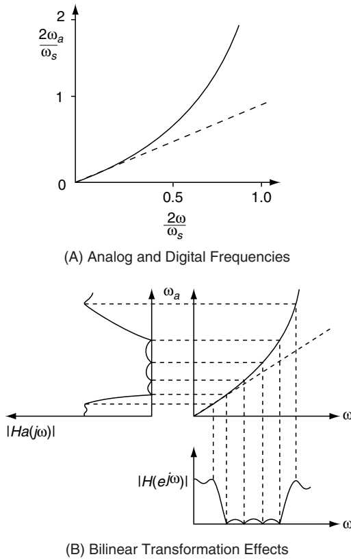
FIGURE 2.21 Bilinear Transformation Warping Effects
