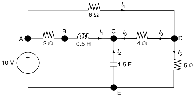
FIGURE 1.2 Example Circuit Diagram
