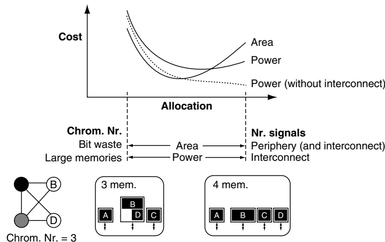
FIGURE 2.23 Exploration Space for the Number of Memories
