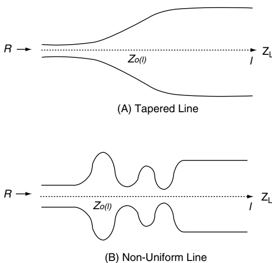
FIGURE 7.12 Tapered Impedance and Non-Uniform Transmission Line Impedance Transformers
