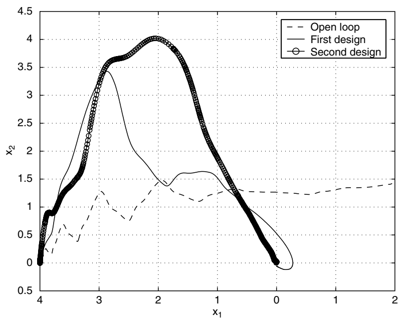
FIGURE 12.3 Direct Adaptive Wing Rock Regulation: Roll and Roll Rate
