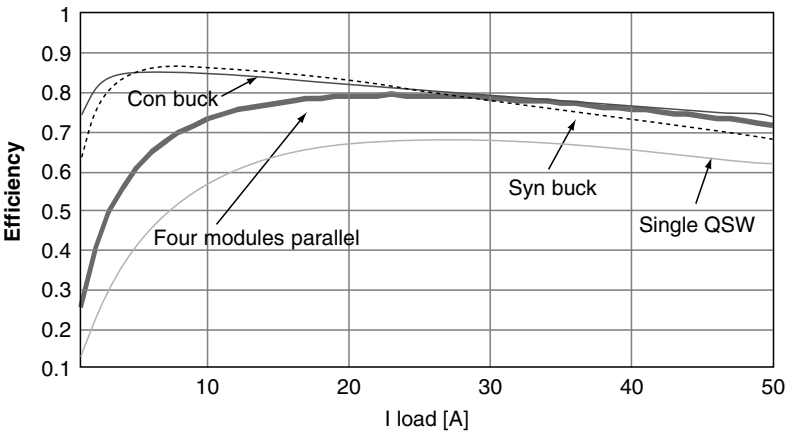
FIGURE 1.19 Efficiency Comparison
