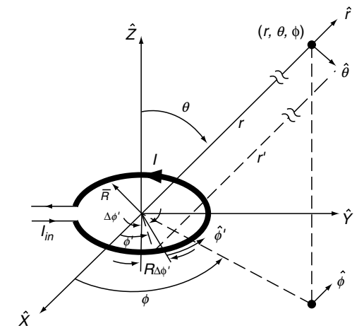
(A) Radiation from a Small Current Loop of Radius R
