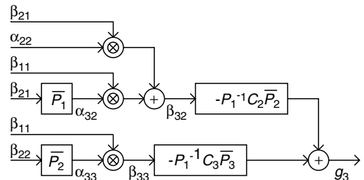
FIGURE 11.4 Simplified G_3 Realization
