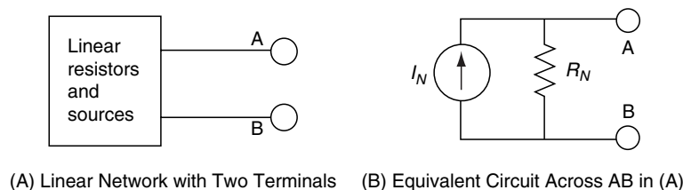
FIGURE 1.16 Norton Equivalent Circuit
