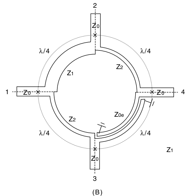
FIGURE 7.19 Two Structure Representations of 180° Hybrid Microstrip Ring Rat-Race Coupler
