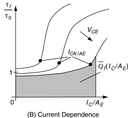
FIGURE 5.8 Bias Dependence of the Forward Transit Time. (A) This graph shows the low-current component for different cases ( V_{C'B'} = V_{CB} ). (B) Notice the current dependence shown here; high-current effects start for I_C > I_{CK} . Typical units: \tau_f in ps; \bar{Q}_f in fC/ \mu\text{m}^2 .
