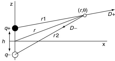
FIGURE 2.5 The Near Cancellation of the Fields of Equal and Opposite Charges Leading to a Far Field that Drops as 1/r^3
