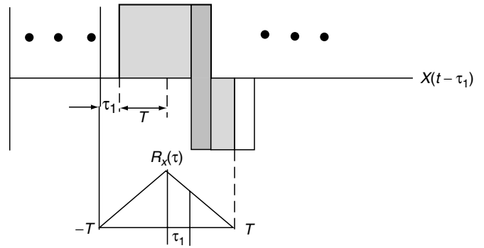
FIGURE 1.5 Autocorrelation Function
