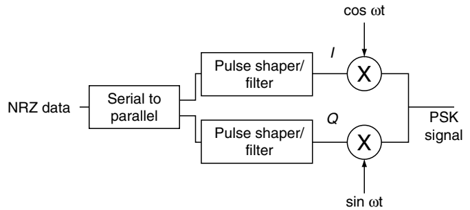
FIGURE 4.3 QPSK Modulator
