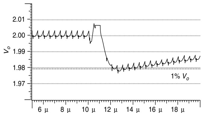
FIGURE 1.35 Transient Response of the Interleaved QSW ( V_{in} = 5 V, V_o = 2 V, and f_s = 1 MHz)
