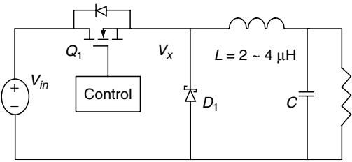
FIGURE 1.3 Conventional Buck Converter
