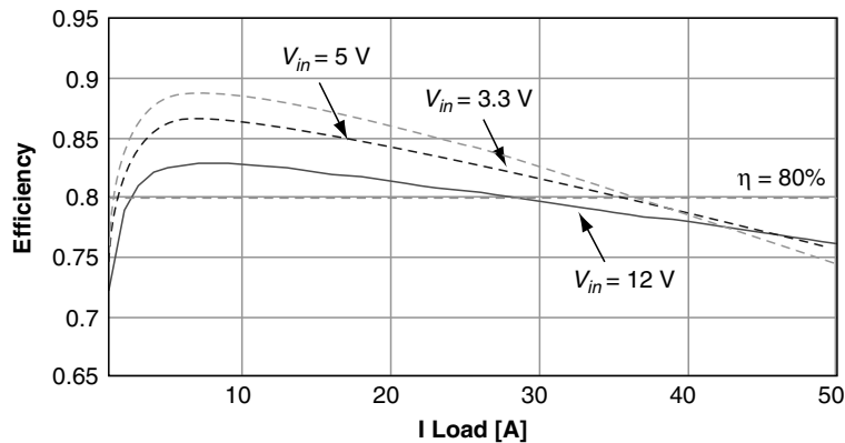
FIGURE 1.25 Efficiency Comparison of Buck Converters ( V_o = 2 V, f_s = 300 kHz, and switches: IRL3803)
