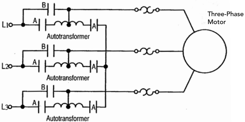
Figure 4.4 Autotransformer Starter
